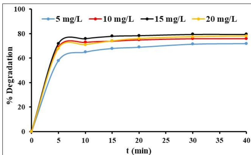
Fig. 4: Effect of \text{Fe}^{2+} concentration on amoxicillin degradation as a function of time, [amoxicillin] = 5 mg/L, [\text{H}_2\text{O}_2] = 100 mg/L, pH=3, T=25°C
