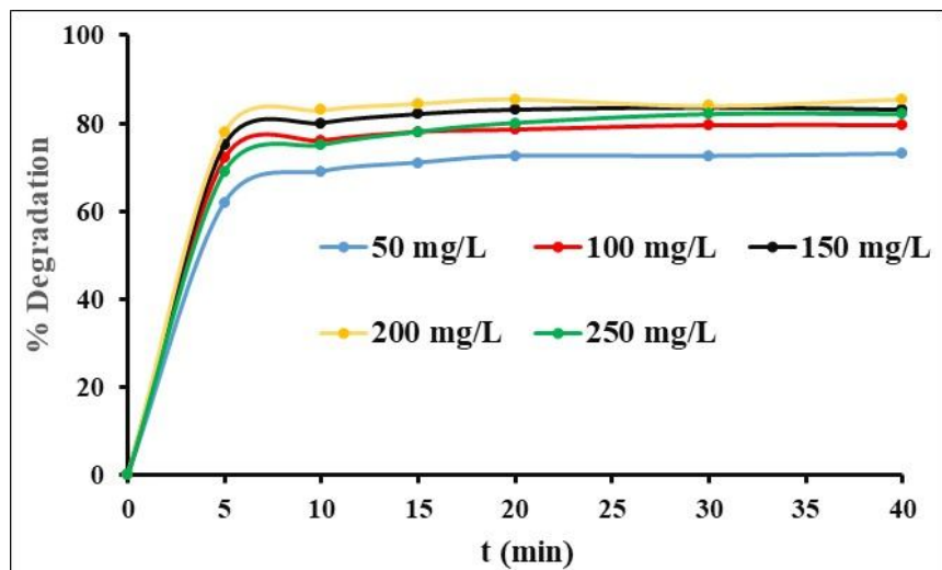
Fig. 5: Effect of H 2 O 2 concentration on amoxicillin degradation as a function of time, [amoxicillin] = 5 mg/L, [Fe 2+ ] = 15 mg/L, pH=3, T=25°C
