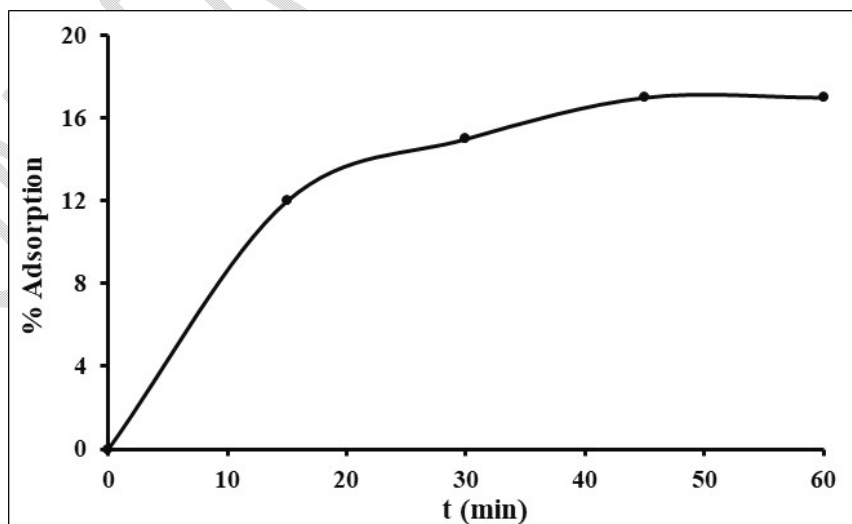
Fig.7: Adsorption rate of amoxicillin on copper oxides as a function of time, [\text{CuO}_x] = 1 \text{ g/L} , [amoxicillin] = 5 mg/L, \text{pH}=3 , T = 25^\circ\text{C}
