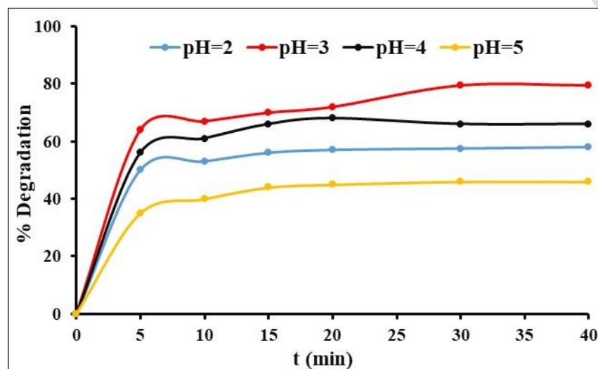
Fig. 2: Effect of pH on amoxicillin degradation as a function of time, [amoxicillin] = 5 mg/L, [\text{Fe}^{2+}] = 15 mg/L, [\text{H}_2\text{O}_2] = 100 mg/L, T=25^\circ\text{C}
