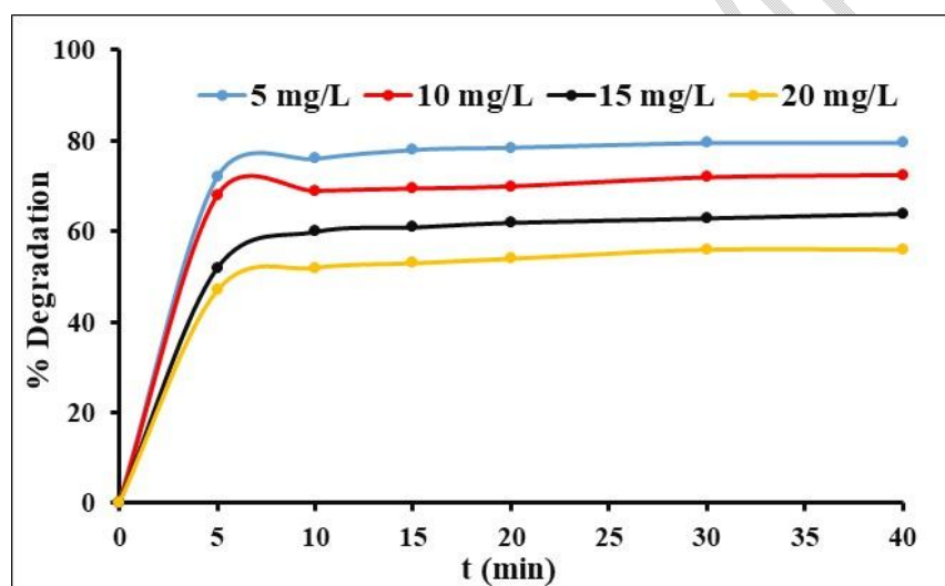
Fig. 3: Effect of amoxicillin concentration on its degradation as a function of time [ Fe^{2+} ] = 15 mg/L, [ H_2O_2 ] = 100 mg/L, pH=3, T=25°C
