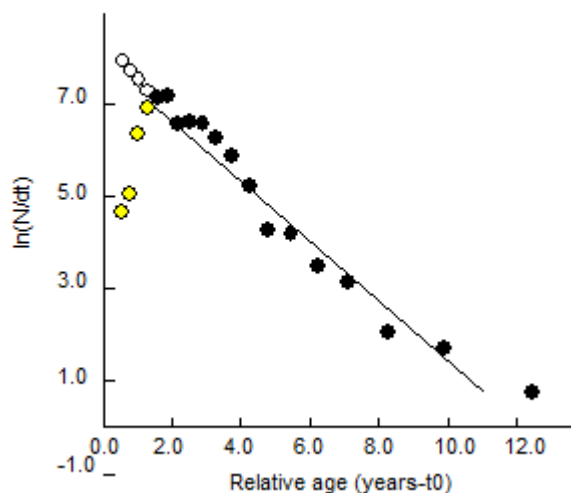
Fig. (3). Von Bertalanffy growth curve (a) ( L_{\infty}=43.05 cm; K = 0.230 \text{yr}^{-1} ); on length-frequency distribution and linearized length-converted catch curve of Nile tilapia in Lake Nubia.
