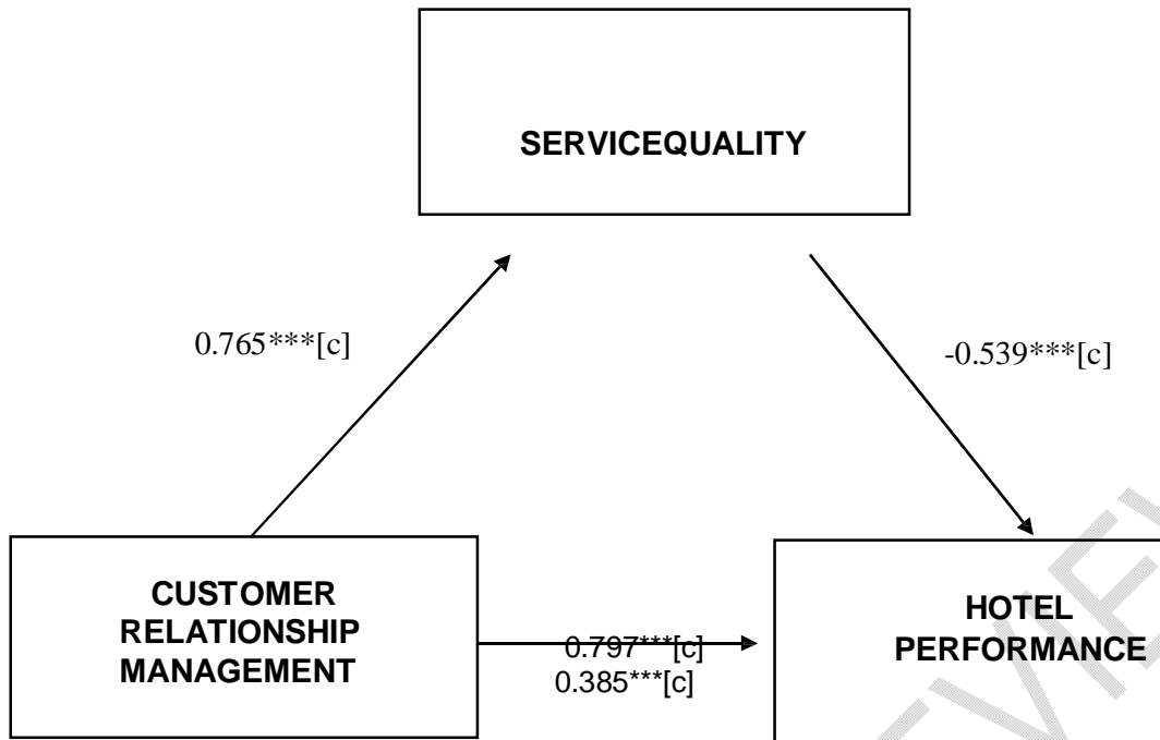
Figure 3. Med graph Showing the Variables of the Study Mediation Analysis of the Three Variables
