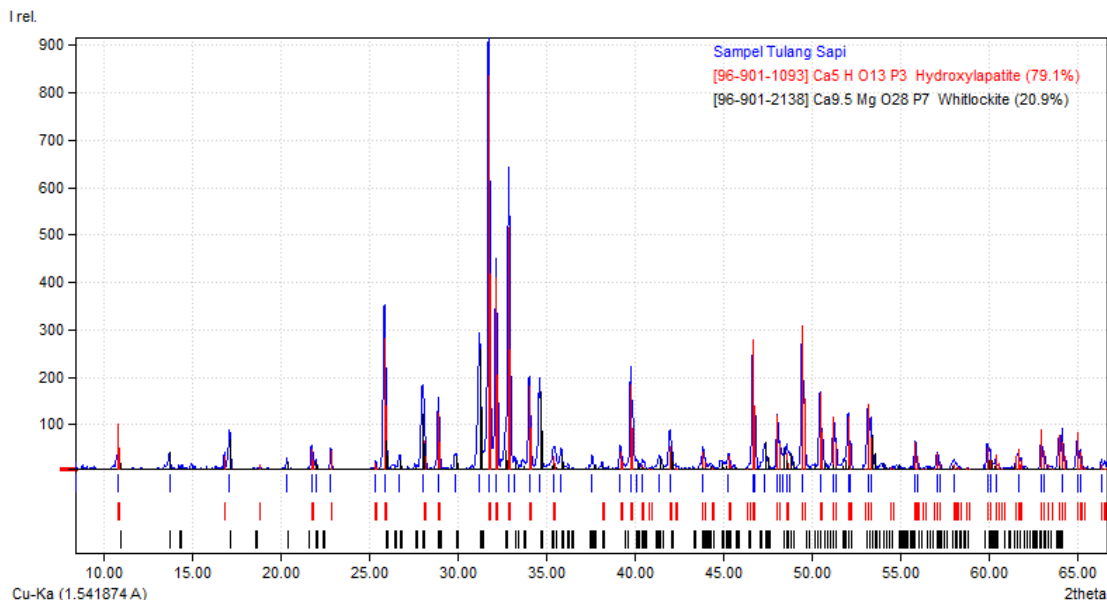
Figure 1. XRD Diffraction Pattern of Hydroxyapatite Produced from CaO Derived from Cow Bones, After Calcination for 10 Hours.
