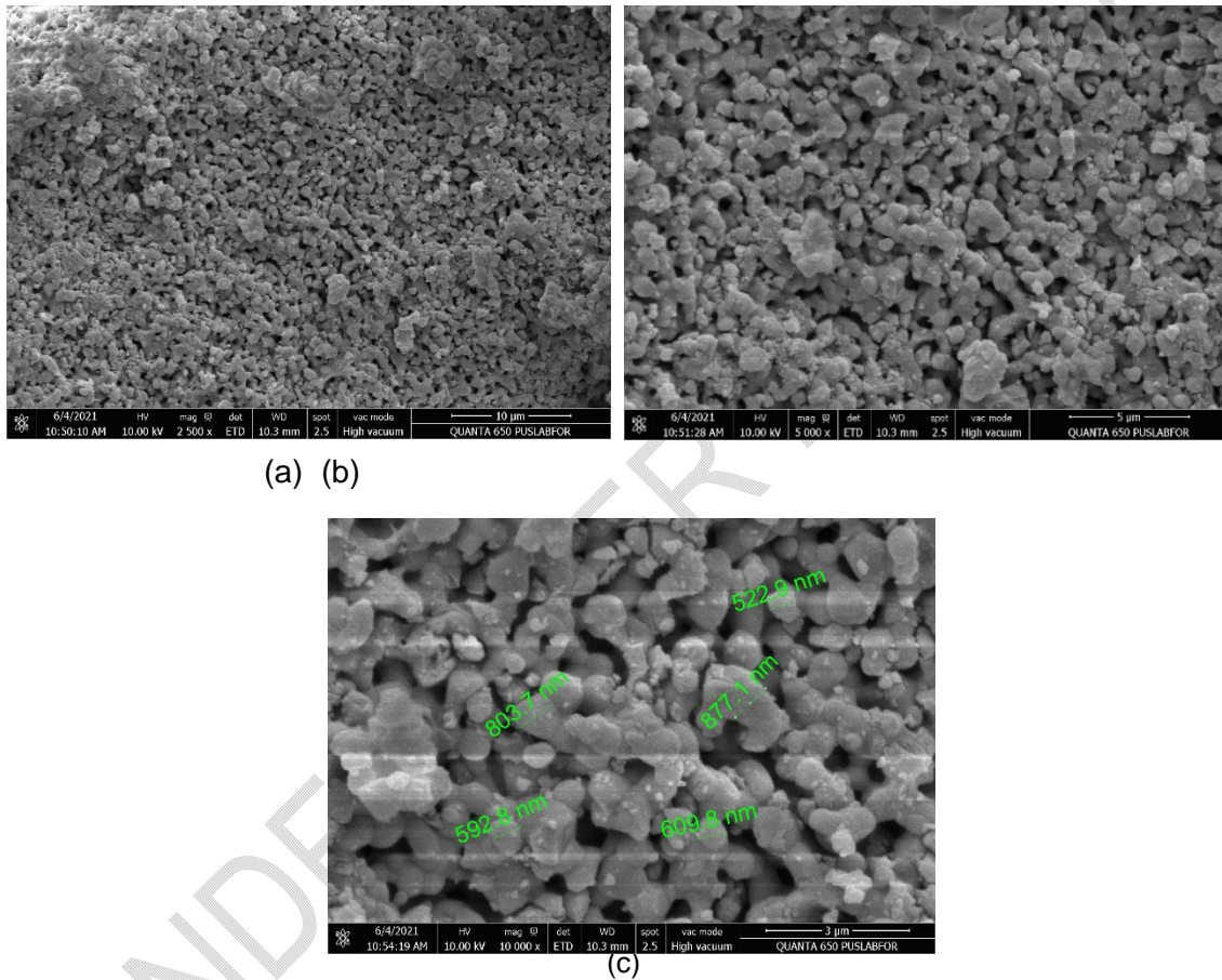
Figure 2. SEM Results of Hydroxyapatite from CaO Source of Cow Bones at Magnifications: (a) 2500x, (b) 5000x, (c) 10000x.
