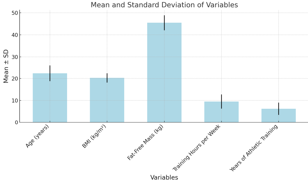
Fig 1: Bar chart representing the mean and standard deviation of the different variables
