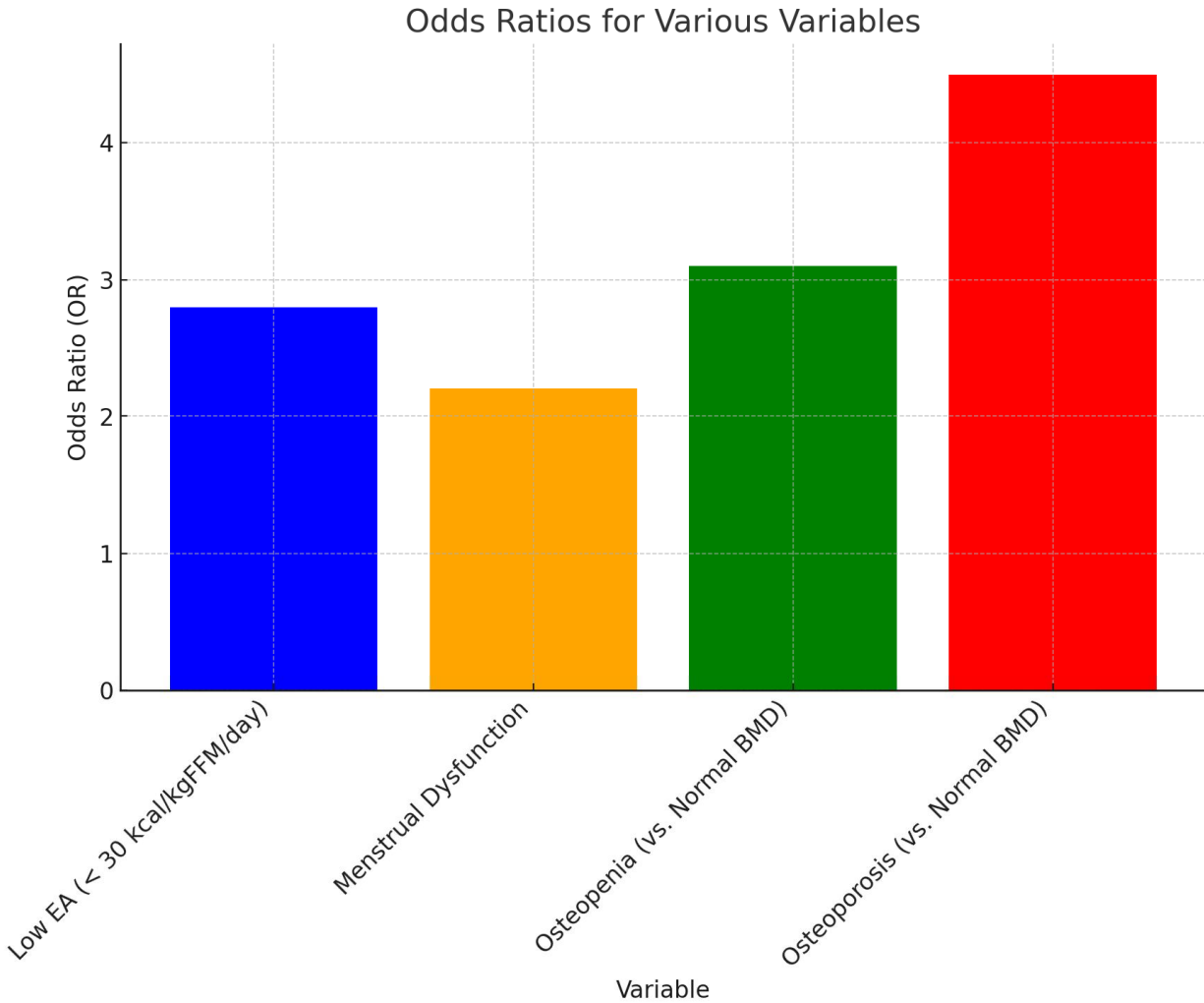
Fig 5: Odds ratios (OR) associated with different variables
