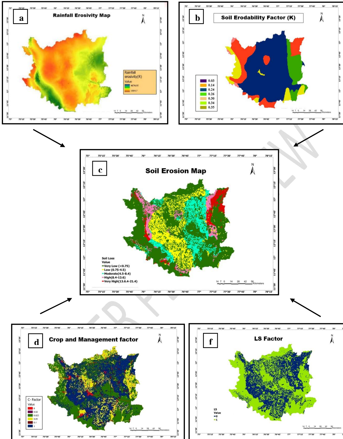
Figure 10. a) Rainfall erosivity map, b) Soil erodibility map, c) Soil erosion map, d) Crop and management factor map, f) Slope length and steepness map
