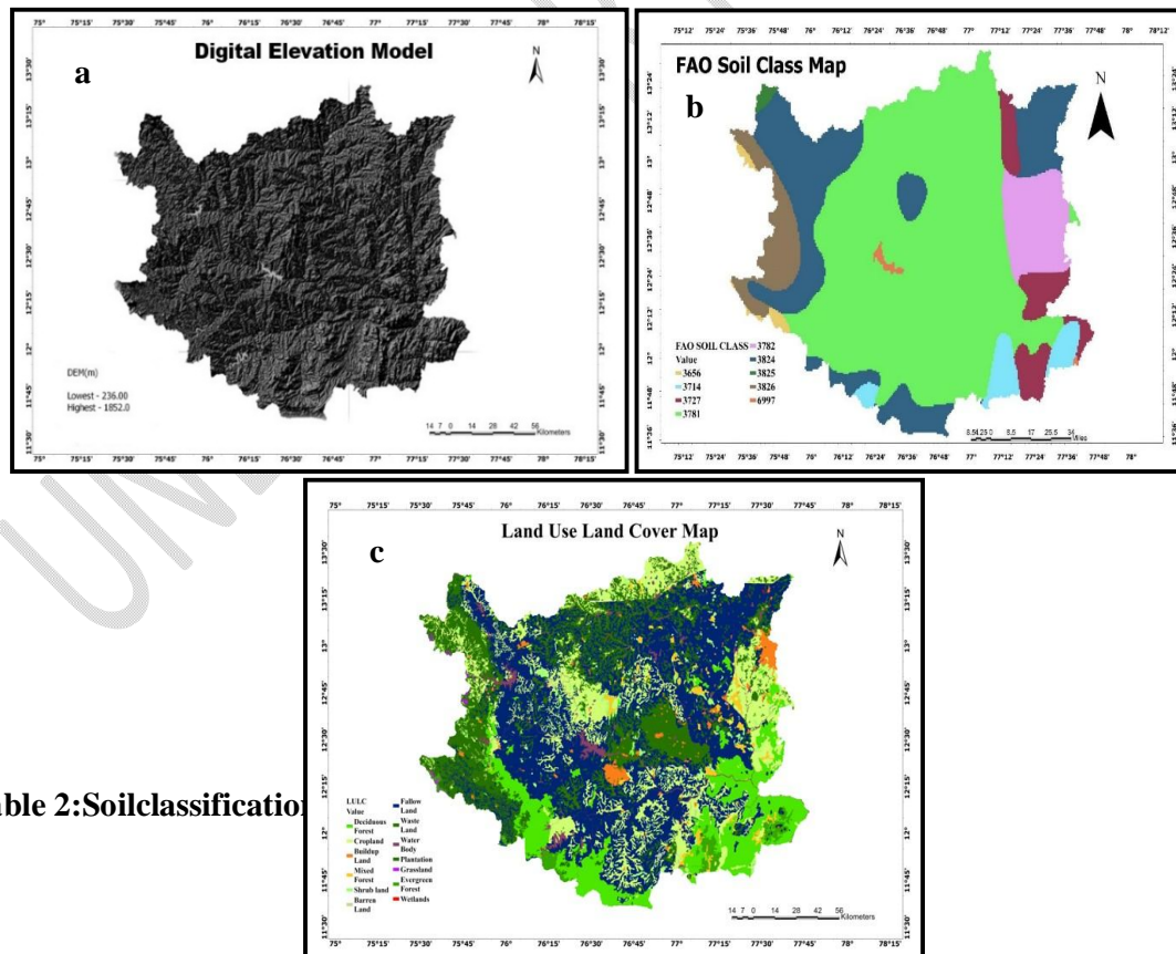
Figure 2: a) Digital elevation model b) Soil classes c) LULC map of the Cauvery River basin
