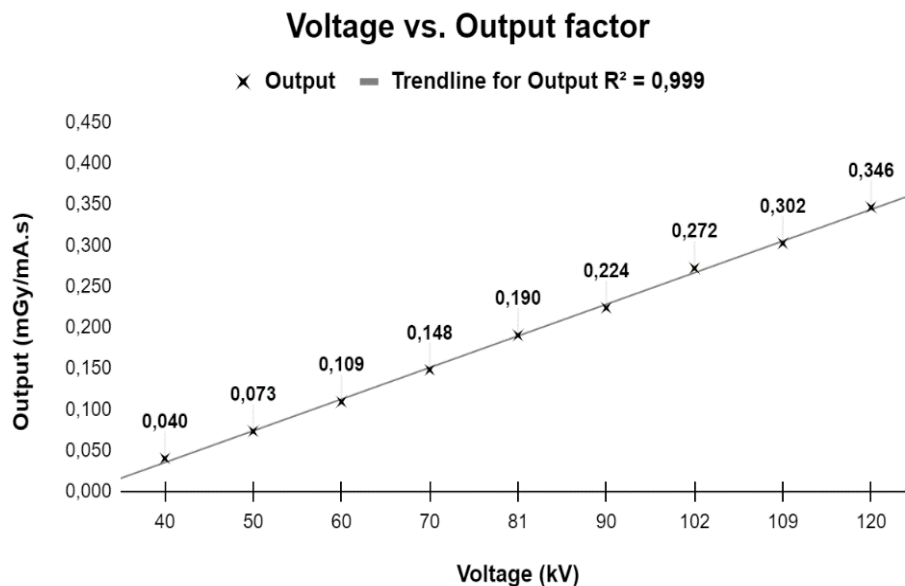
Fig. 3. The output curve of the radiographic tube
