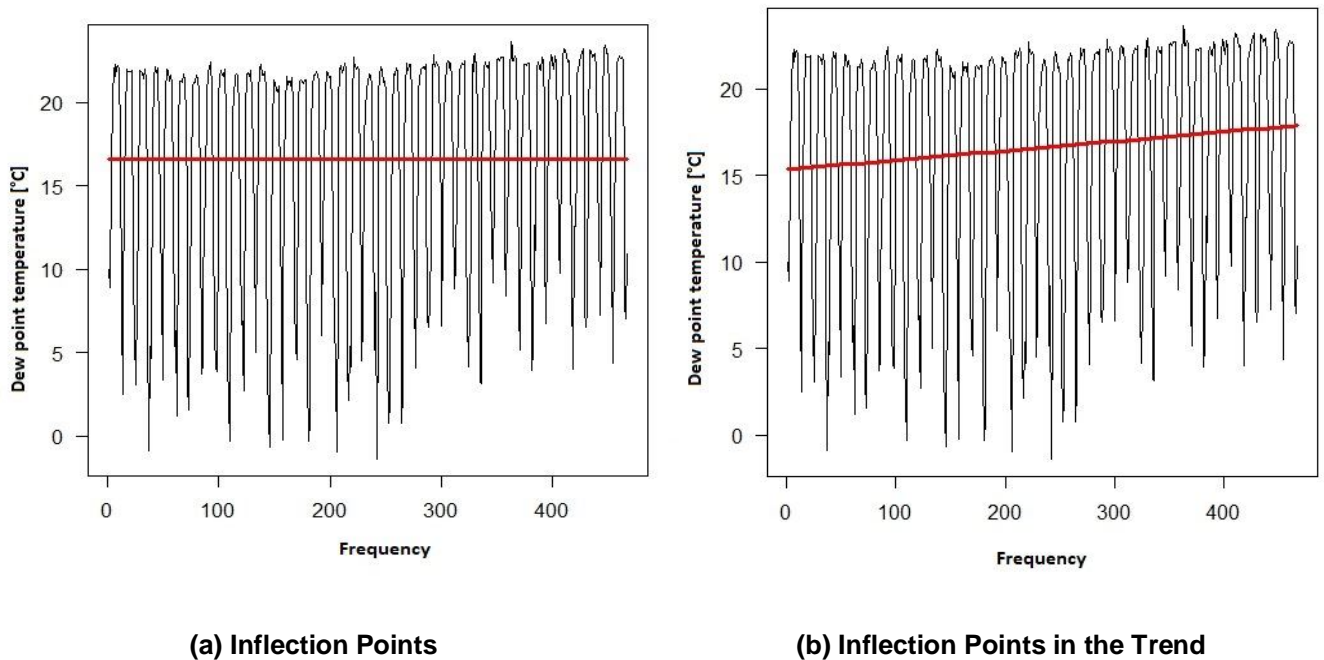
Fig. 8. Identification of inflection points in the distribution of dew point temperature data
