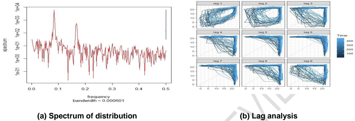
Fig. 9. Spectrum and lag plots of dew point temperature data distribution
