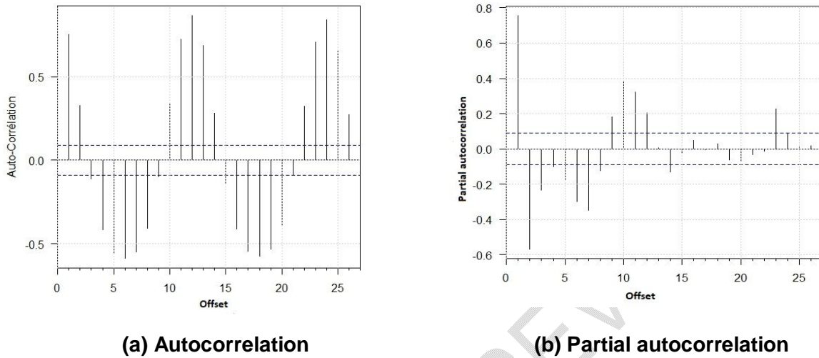
Fig. 7. Estimation of autocorrelation function for distribution of dew point data
