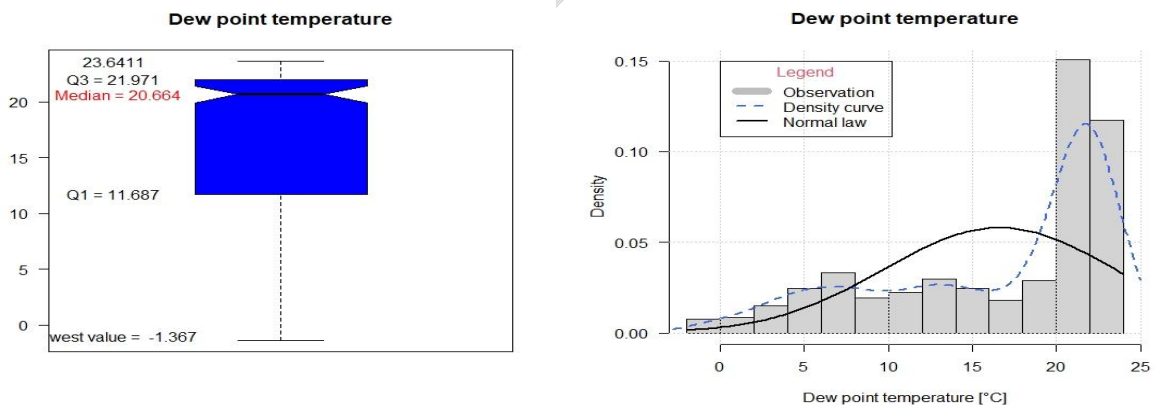
Fig. 2. Analysis of distribution of dew point temperature data
