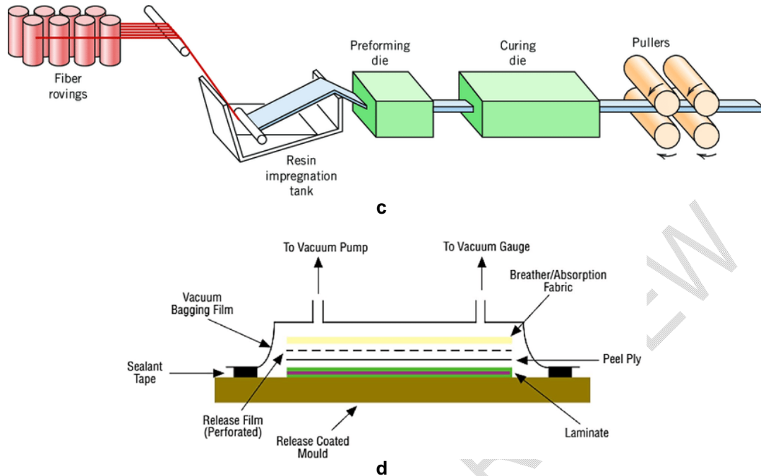
Fig. 1 Manufacturing process techniques a) Hand lay-up Process b) Filament winding Process, c) Pultrusion Process d) Vacuum-assisted Process
