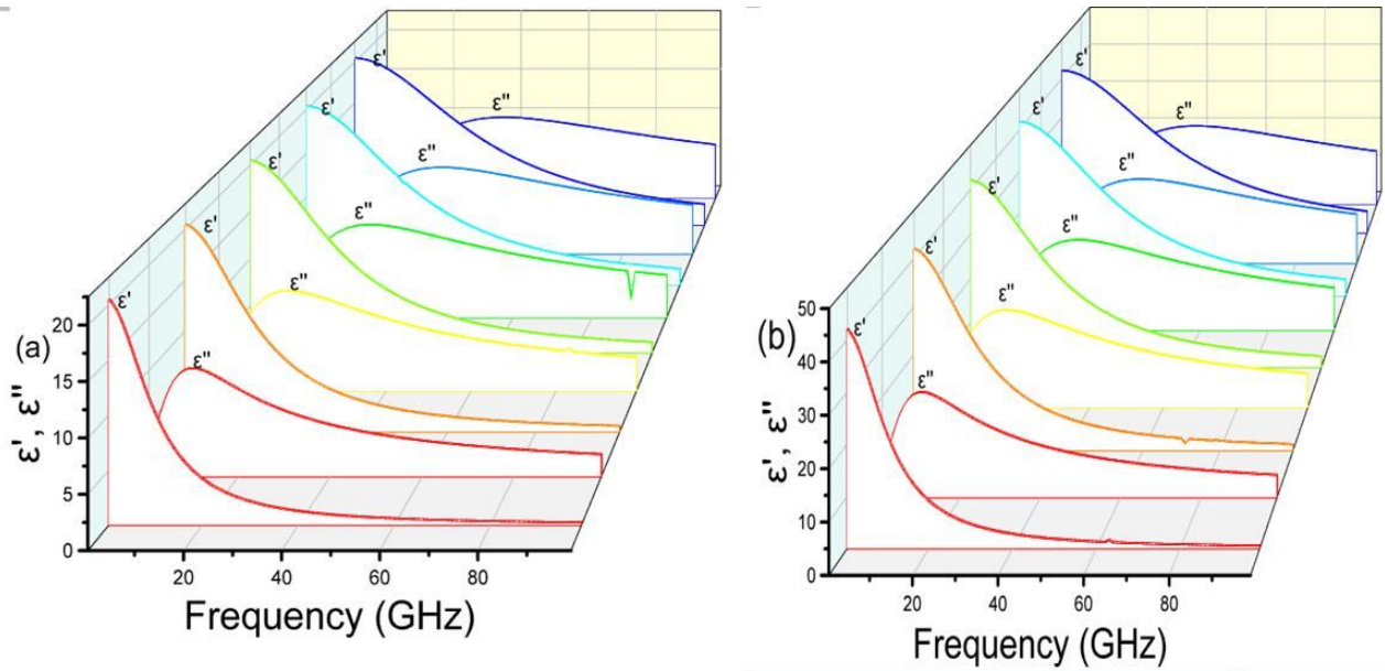
Figure 7: Frequency dependency of the dielectric constant ( \epsilon' ) and loss factor ( \epsilon'' ) of (a) Graphene and (b) G4/T10/PVDF
