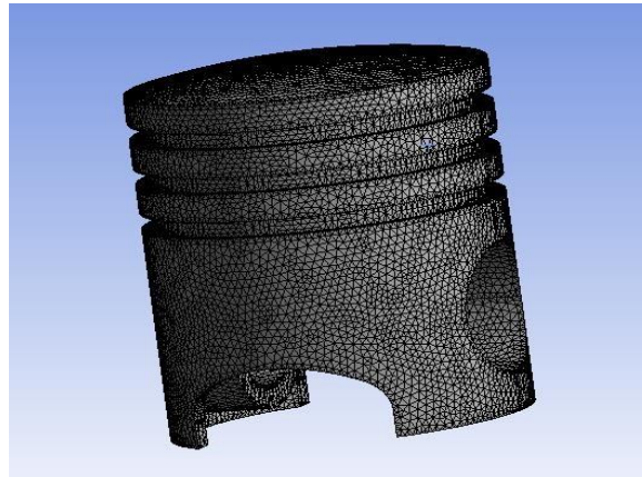
Fig. 3.Mesh: nodes:188577 element:105885
