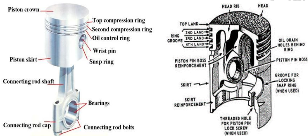
Fig. 1. Simple construction of a piston (Manjunatha, 2013).
