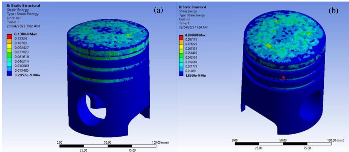
Fig. 10. Strain energy of (a) Al6061 and (b) AISiC
