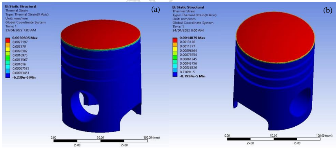
Fig. 11. Thermal strain of Al6061 and AISiC
