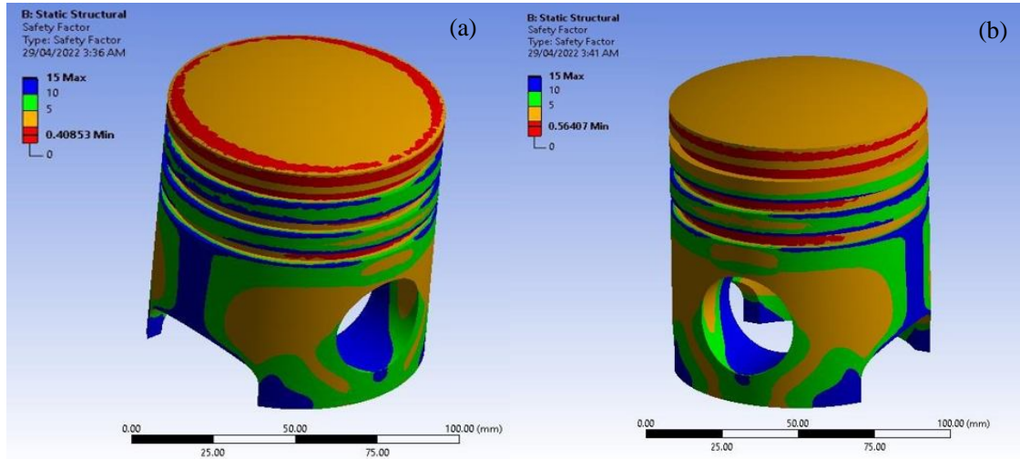
Fig. 12. Factor of Safety of (a) Al6061 and (b) AlSiC
