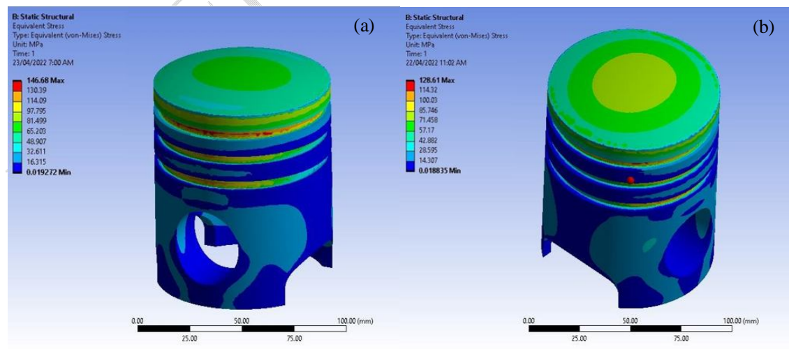
Fig. 9. Equivalent (Von-Mises) stress of (a) Al6061 and (b) AISiC
