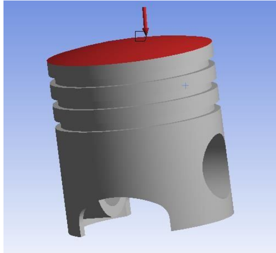
Fig. 4. Structural boundary condition (Pressure)
