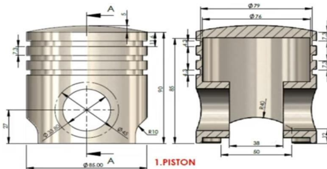
Fig. 2. Basic dimensions of the piston.
