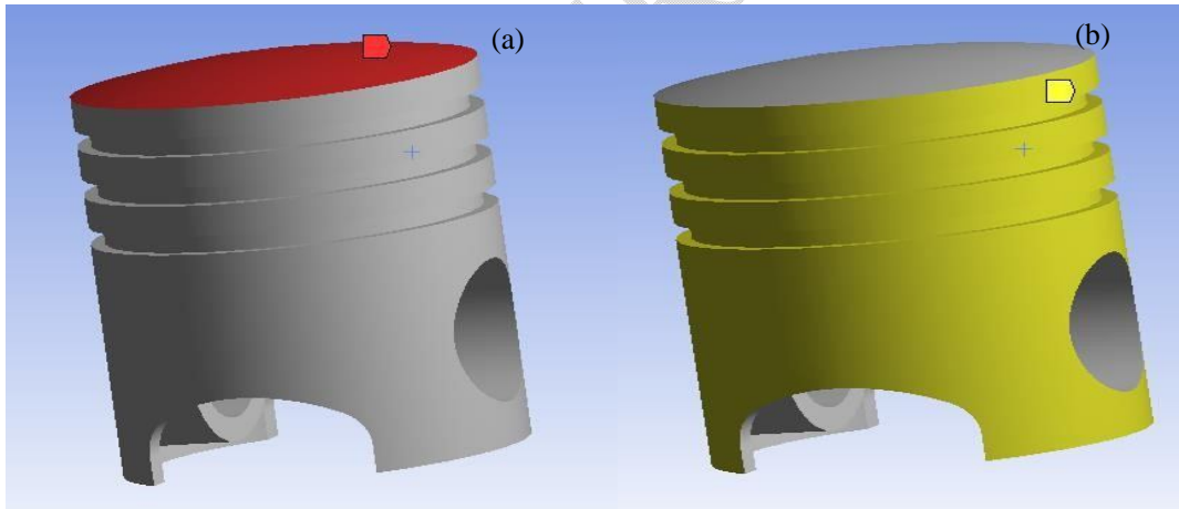
Fig.5. Thermal boundary conditions: (a) temperature and (b) convection of the material
