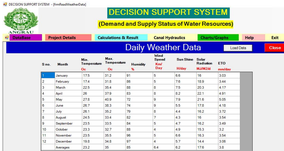
Fig. 3. Mean monthly weather data of command
