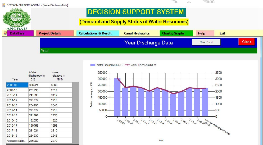
Fig.4. Annual mean discharge at command area during 2008-09 to 2018-19
