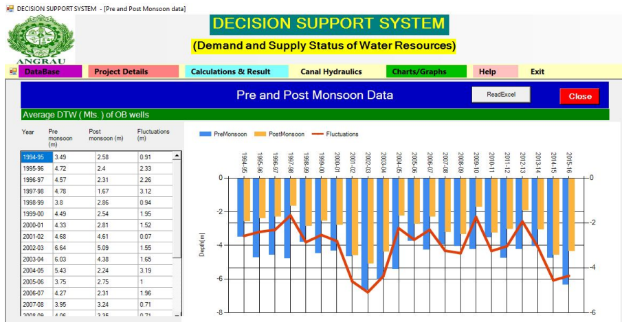
Fig. 5. Pre and Post monsoon data at NSP command area from 1994-95 to 2015-16
