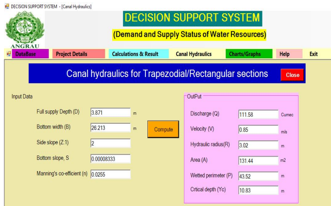
Fig. 13. Computation of discharge of canal
