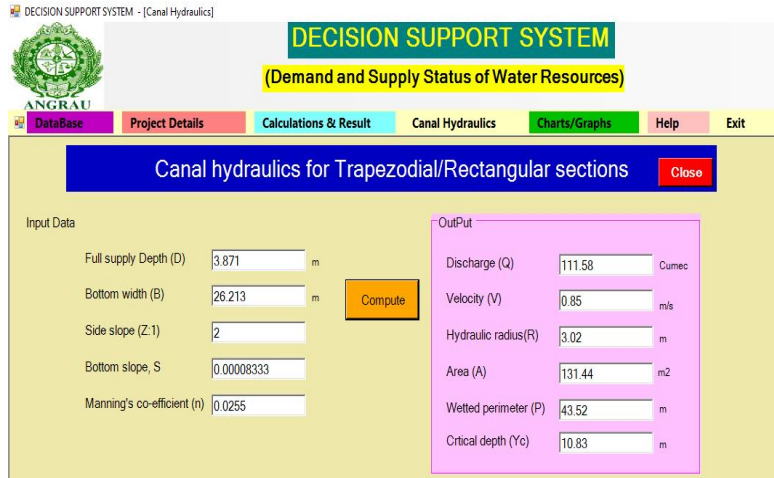
Fig. 13. Computation of discharge of canal
