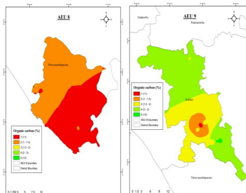
Fig 2: Spatial distribution of soil organic carbon of AEU 3, 4, 5, 8 and 9
