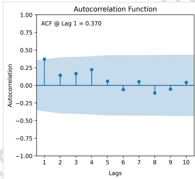
Figure 3: Rainfall correlogram of ACF for Umuahia
