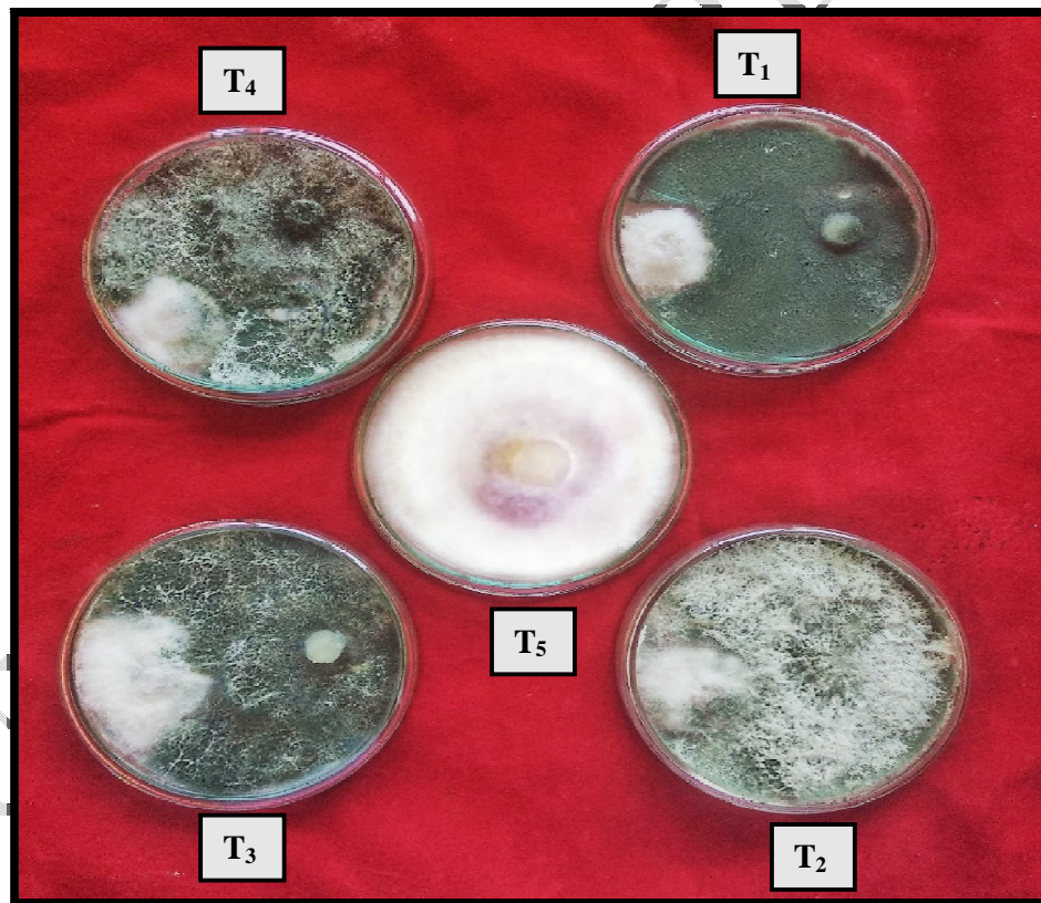
Plate 2: In vitro efficacy of bioagents against Fusarium oxysporum f. sp. niveum .
