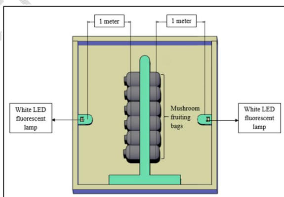
Figure 1. Perspective view of mushroom cultivation room.
