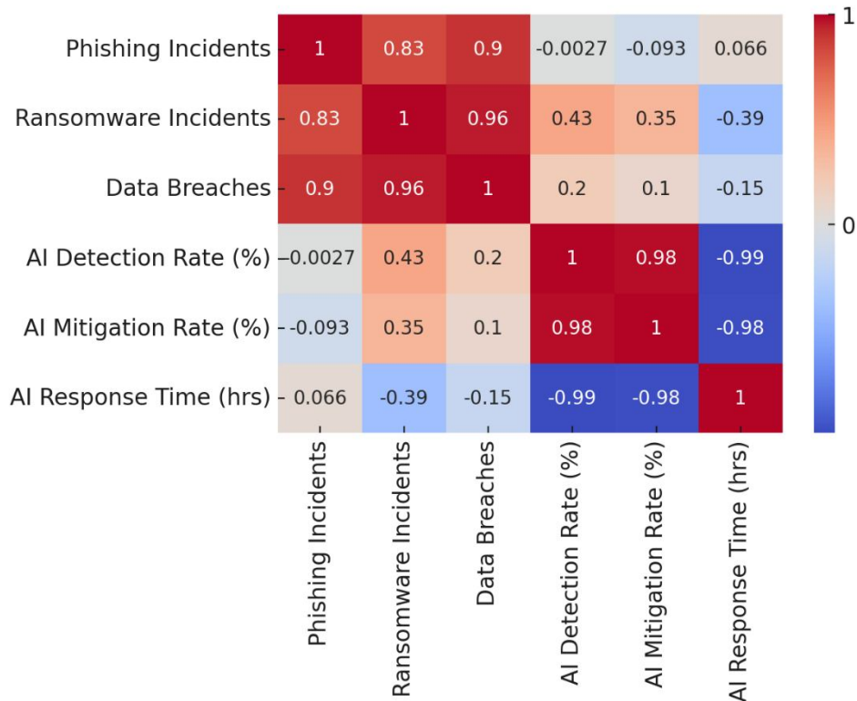
Figure 7: Correlation Matrix:
