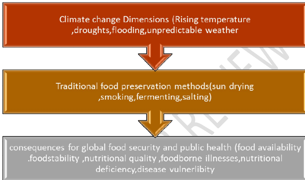
Fig 1: Study Protocol
