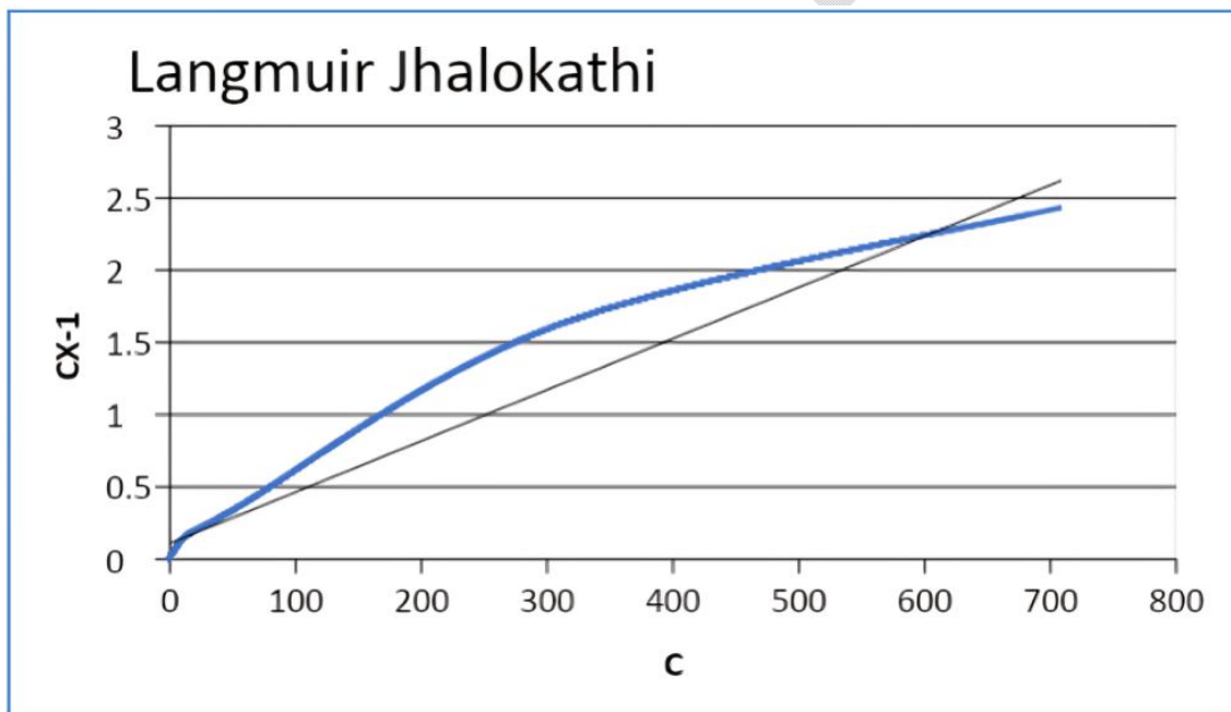
Fig. 8: Langmuir adsorption isotherm for phosphorus in Jhalokathi soil series
