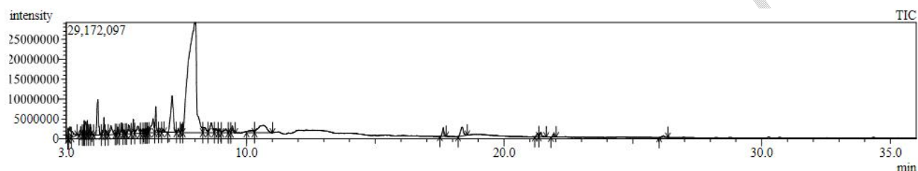
Fig 1b. GC/MS chromatogram of methanol extract of Crunchy kernel of Borassusflabellifer L.
