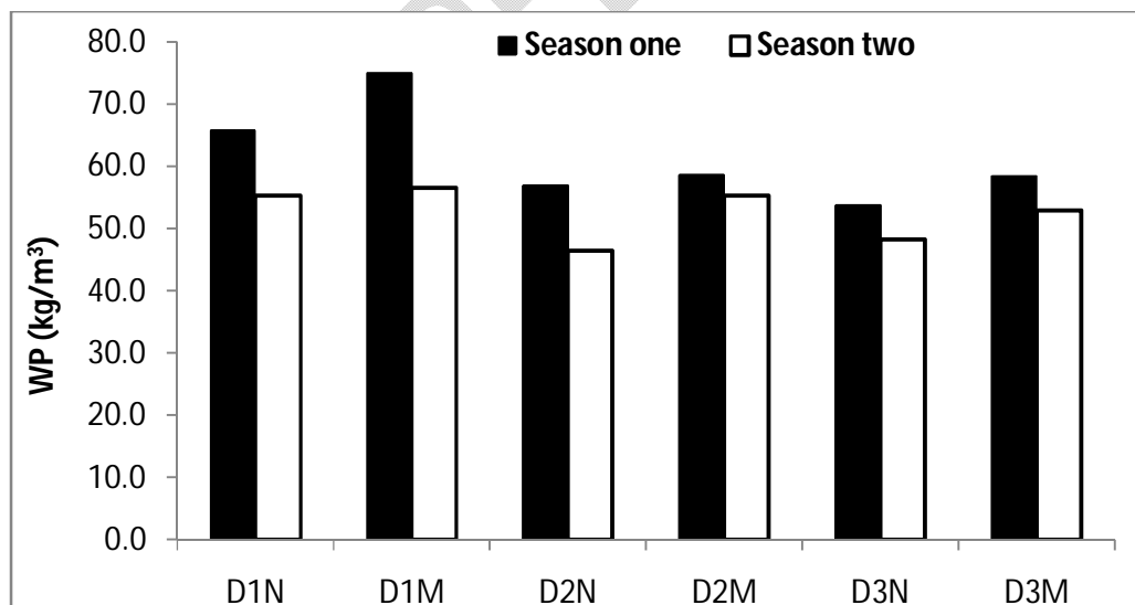
Figure 1. Effect of drip irrigation regimes and mulching on water productivity (WP) of cucumber grown under greenhouse conditions.
