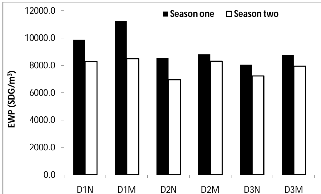
Figure 2. Effect of drip irrigation regimes and mulching on economic water productivity (EWP) of cucumber grown under greenhouse conditions.
