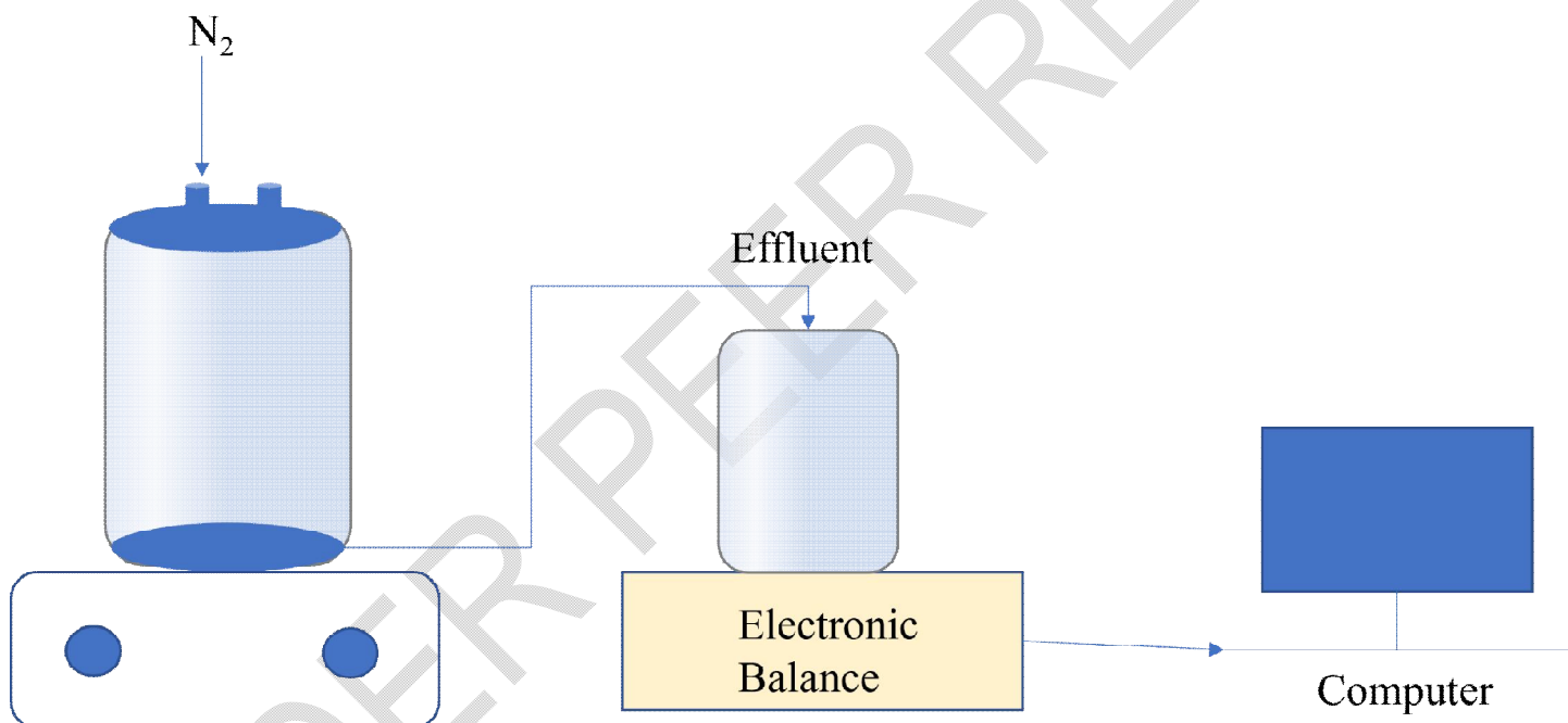
Fig.1. Diagram of ultrafiltration experimental setup.
