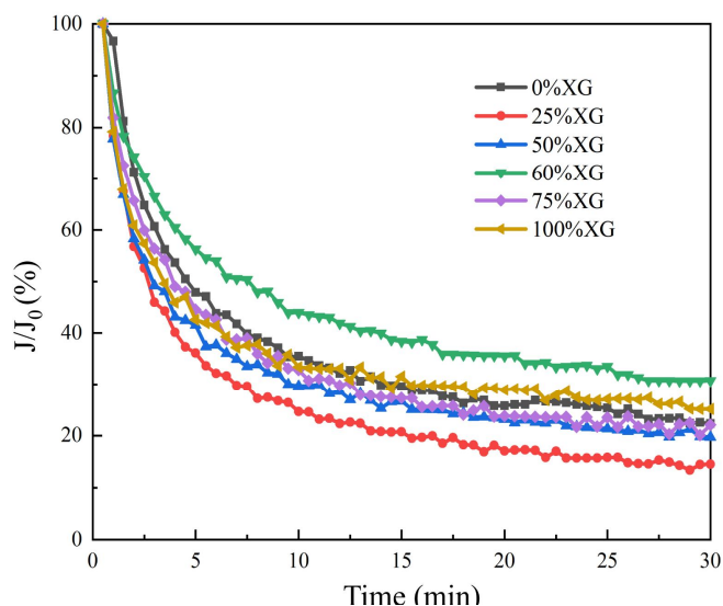
Fig. 2. Membrane flux attenuation of nZVI/PVDF modified membrane for filtering simulated water samples with different xanthan gum content
