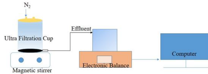
Fig.1. Diagram of ultrafiltration experimental setup.
