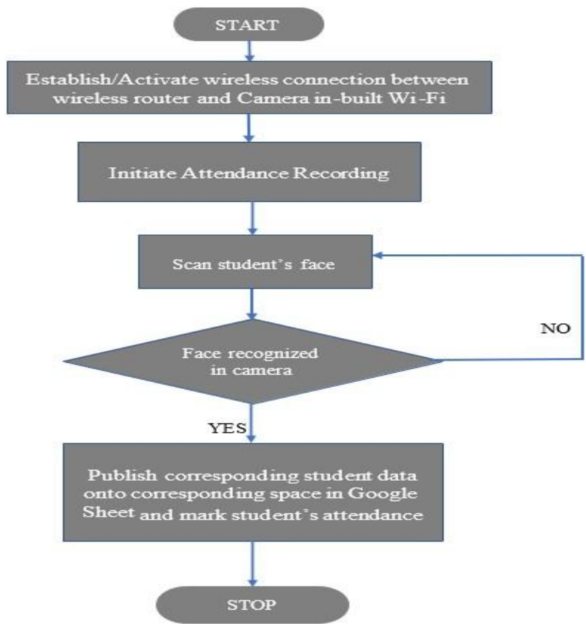
Figure5:Flow chat of thefacerecognition-based attendancesystem.
