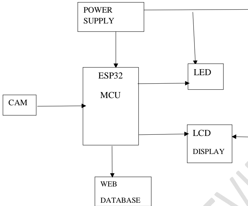
Figure1: System Block Diagram of the face recognition-based attendancesystem.
