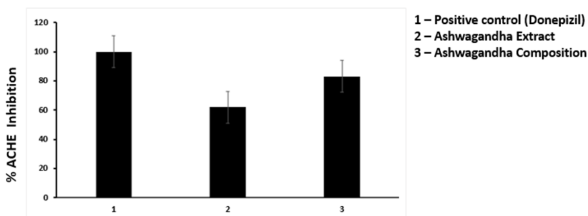
Figure 3: Graph representing the percentage of Acetylcholinesterase inhibition for W. somnifera extract and Composition
