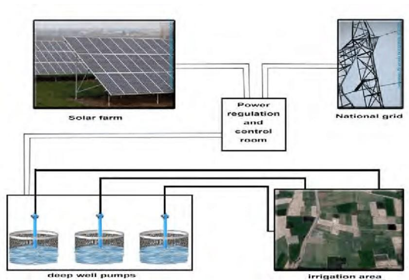
Figure 1: Schematic Diagram of a Solar-powered Irrigation System
