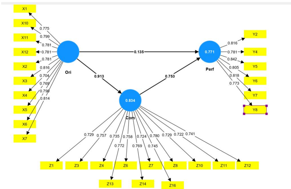
Figure 2. Path diagram model
