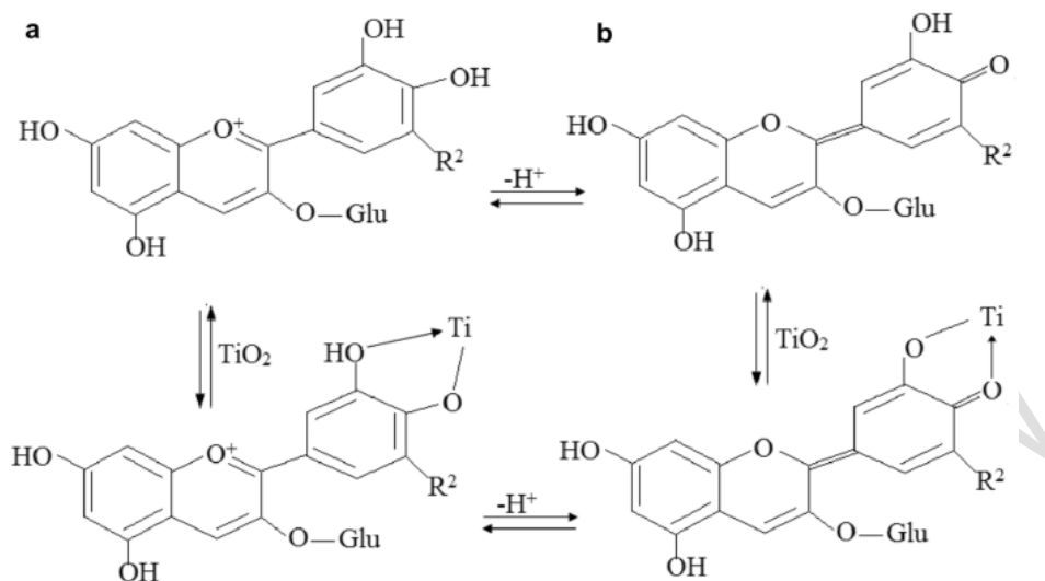
Fig 6. Schematic representation of the interaction between cyanidine-3-glucoside (anthocyanin) and \text{TiO}_2 [130].
