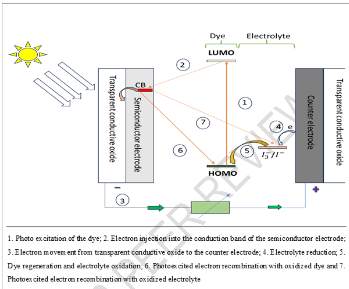
Fig 1. Structure and operation of a dye-sensitized solar cell.
