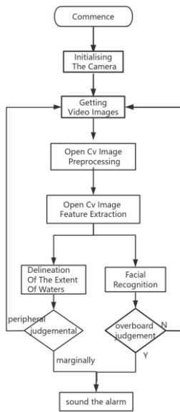
Fig. 4. Detection module programme flow chart
