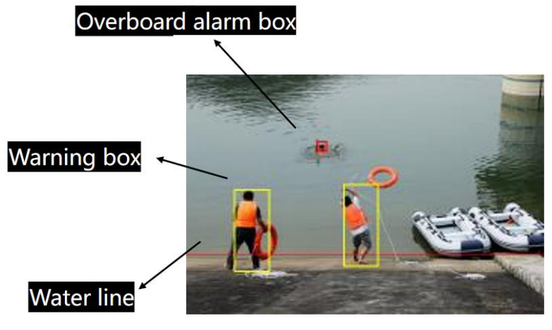
Fig. 5. Detection effect chart
