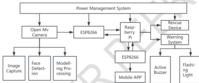
Fig. 2 .Schematic diagram of system hardware design
