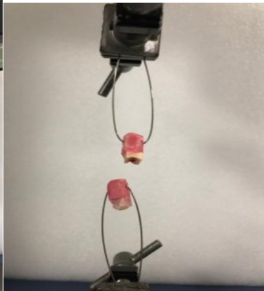
Fig 13: Sample subjected to Microshear stress
