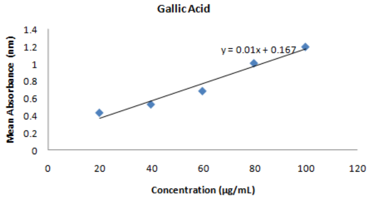
Figure 16. Total phenolic content for standard gallic acid
