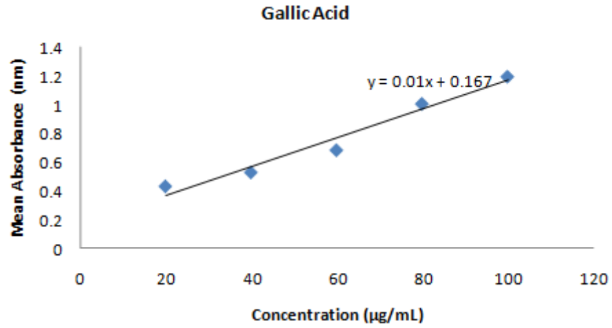
Figure 16. Total phenolic content for standard gallic acid
