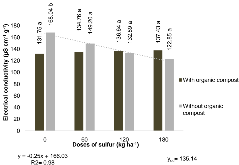
Figure 2. Electrical conductivity of radish seeds as a function of the sulfur doses in top dressing with organic compost ( y_{oc} ) and without organic ( y ) and averages with and without organic compost for each dose of sulfur.
