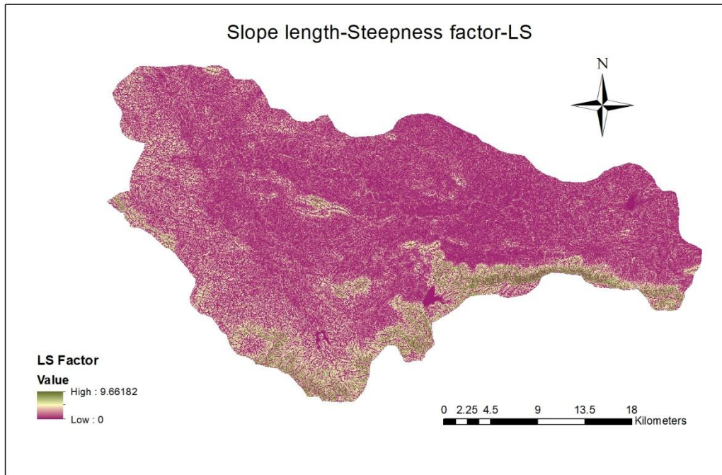
Figure 5. Slope length and steepness factor (LS Factor) map.
