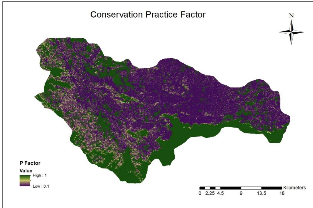
Figure 9. Conservation practice factor (P Factor) map.
