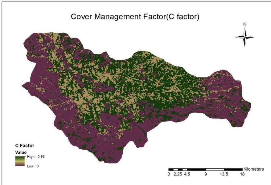
Figure 7. Cover management factor (C Factor) map.
