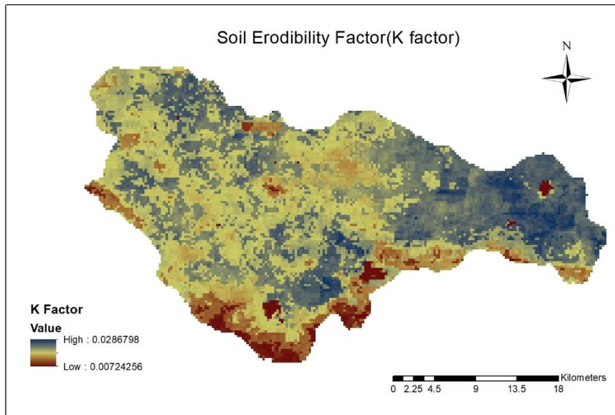
Figure 4. Soil erodibility factor(K Factor) map.
