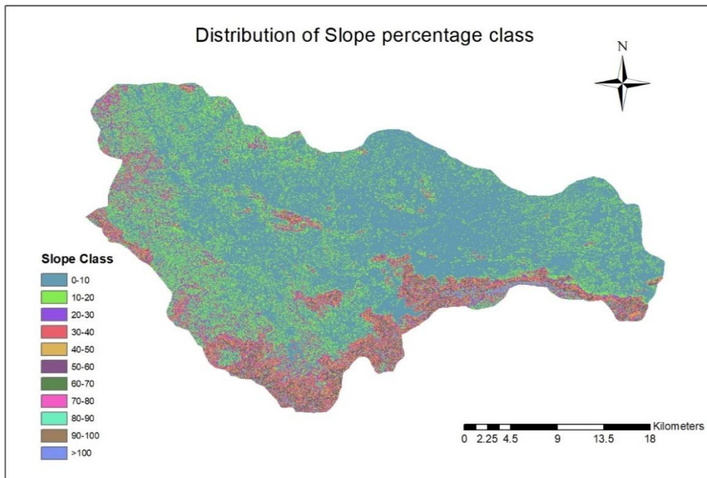
Figure 6. Distribution of slope class in the study area.
