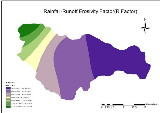
Figure 3. Rainfall-runoff erosivity factor (R Factor) Map
