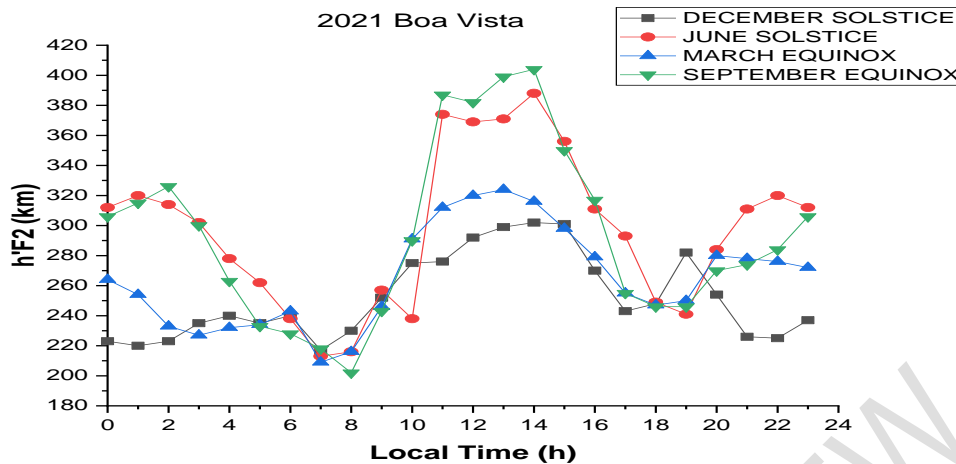
Fig. 4: Diurnal and seasonal variation of h'F2 at Boa Vista station during ascending phase of solar cycle 25
