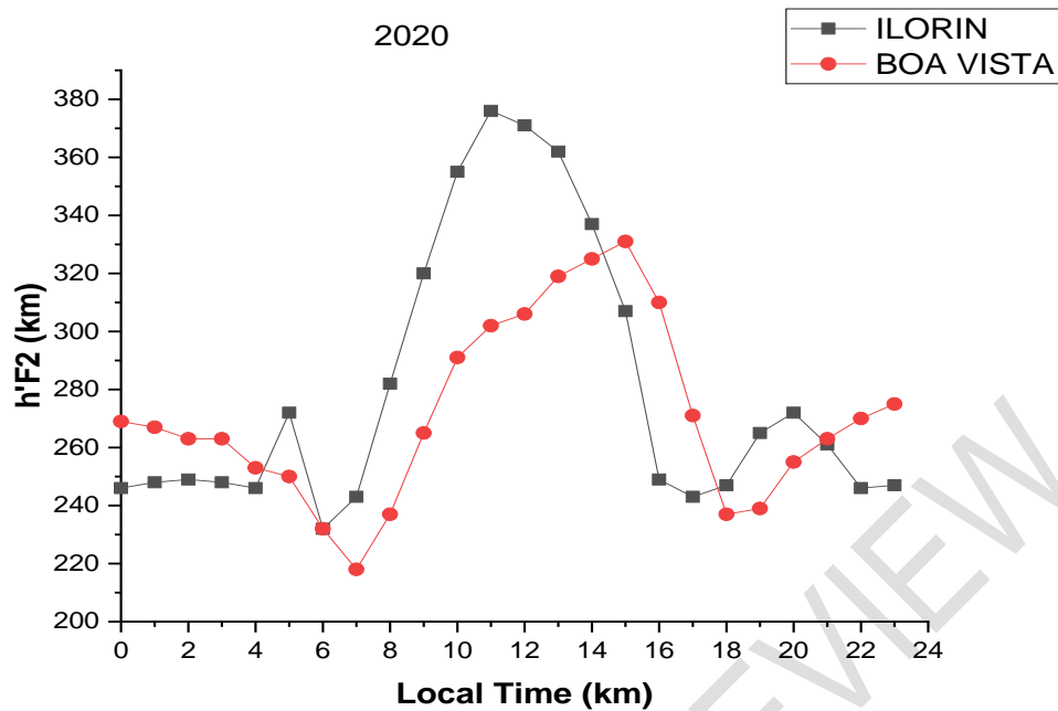
Fig. 5: Annual Variation of h'F2 at Ilorin and Boa Vista during minimum phase of solar cycle 25
