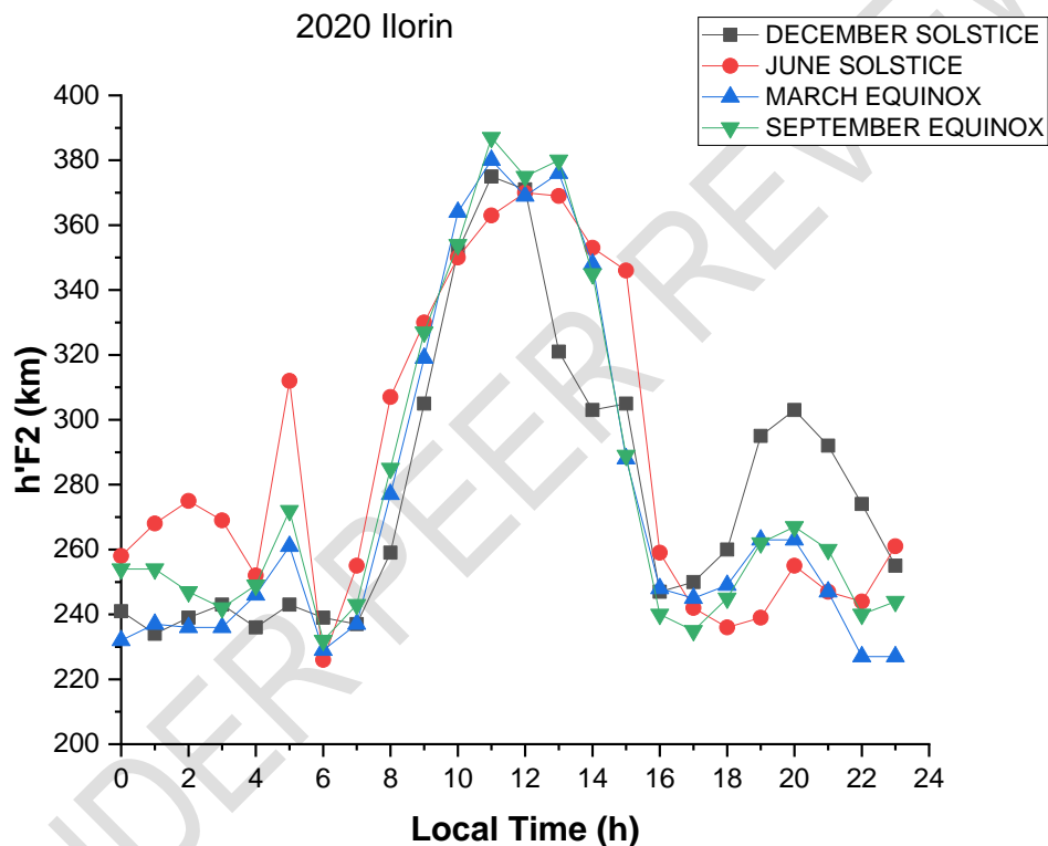
Fig. 1: Diurnal and seasonal variation of h'F2 at Ilorin during minimum phase of solar cycle 25
