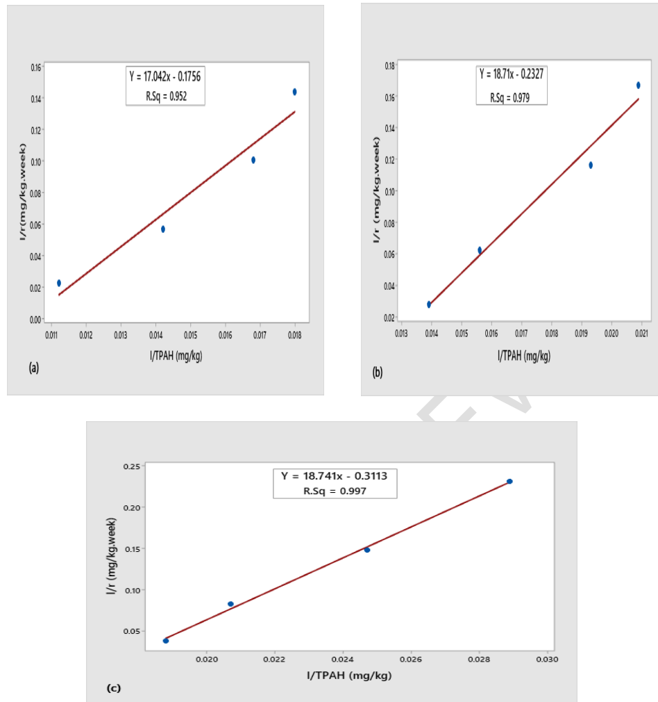
Figure 5: Lineweaver-Burk plot for TPAH for SEO - Contaminated Soil Treated with; (a) 250g of BLE (b) 500g of BLE and (c) 750 BLE
