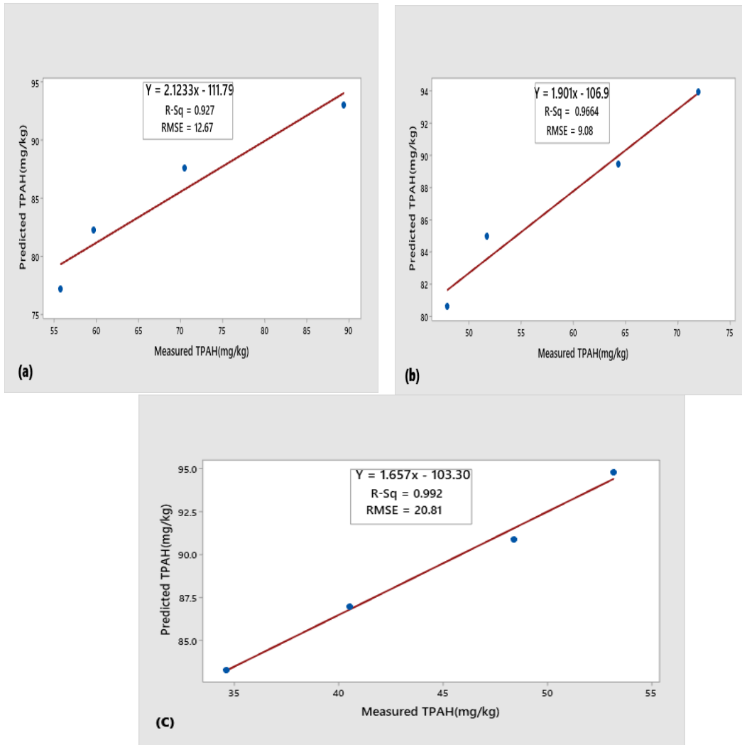
Figure 6: Predicted vs measured TPAH for SEO - Contaminated Soil Treated with; (a) 250g of BLE (b) 500g of BLE and (c) 750 BLE
