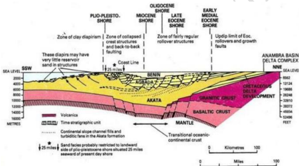
Figure 2. Niger Delta Stratigraphy Sequence
