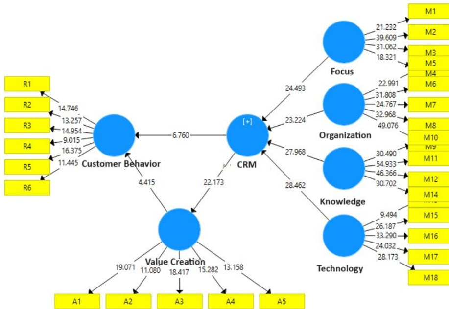
Figure 1: Tested Model of Research Variables (Path Coefficients)
