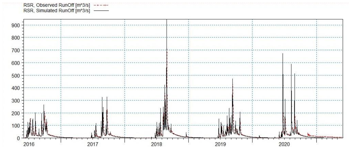
Figure 13: Observed and simulated runoff hydrograph during model validation
