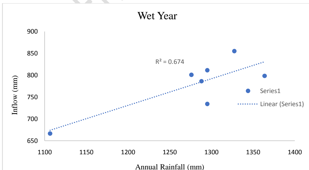
Figure9: Linear relation between rainfall and runoff in wet years
