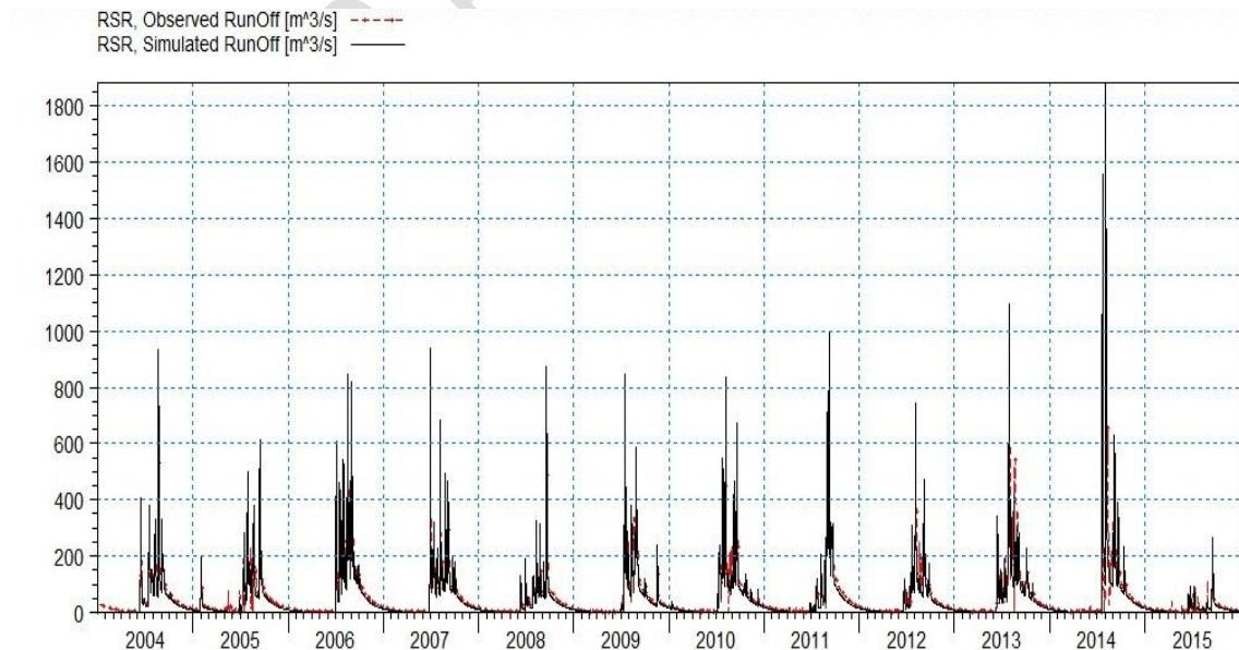
Figure 11: Observed and simulated runoff hydrograph during model calibration
