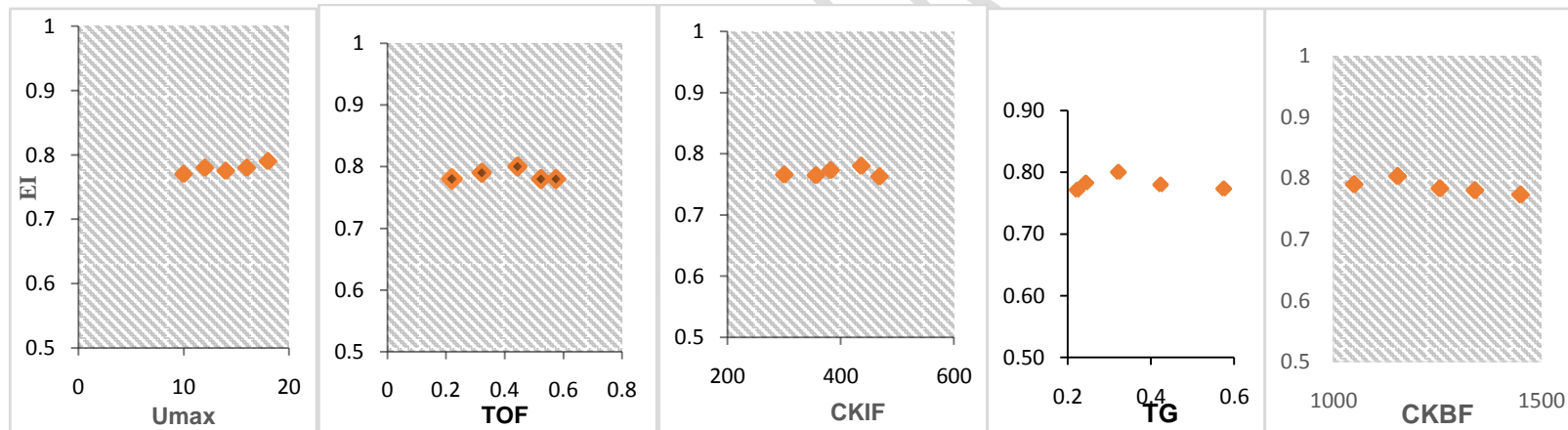
Figure 16: Graph between EI against the sensitive model parameter
