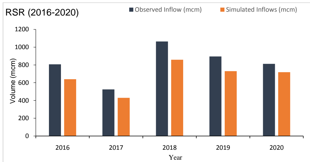
Figure14:ObservedandsimulatedrunoffhydrographduringmodelValidation
