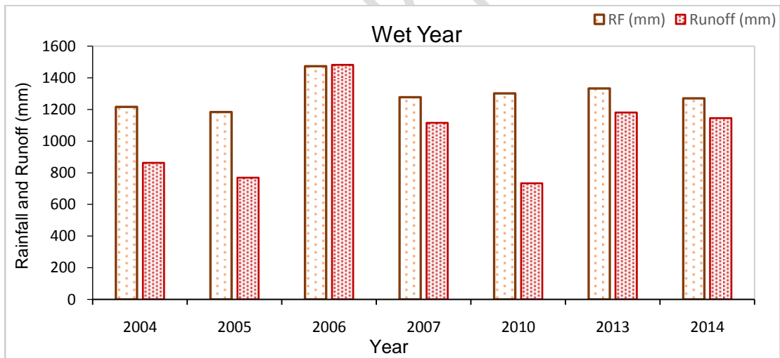
Figure7: Annual Runoff of Study Area in during wet year
