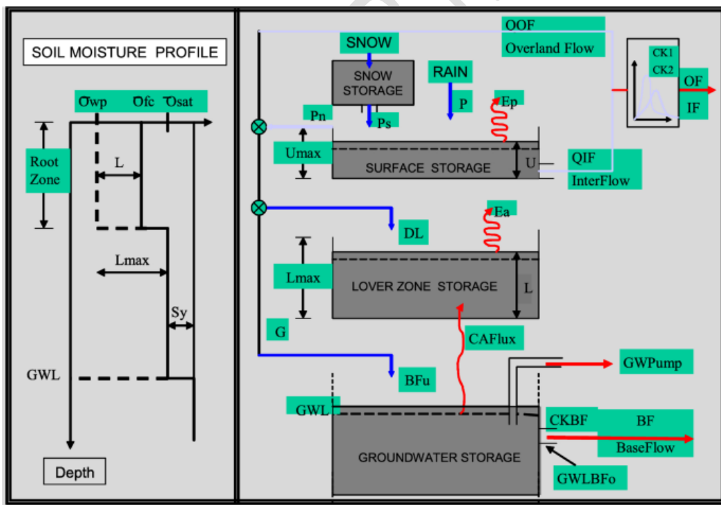
Figure2: Structure and Processes of NAM Model
