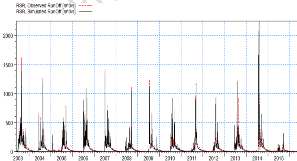
Figure 11:Observedandsimulatedrunoffhydrographduringmodelcalibration
