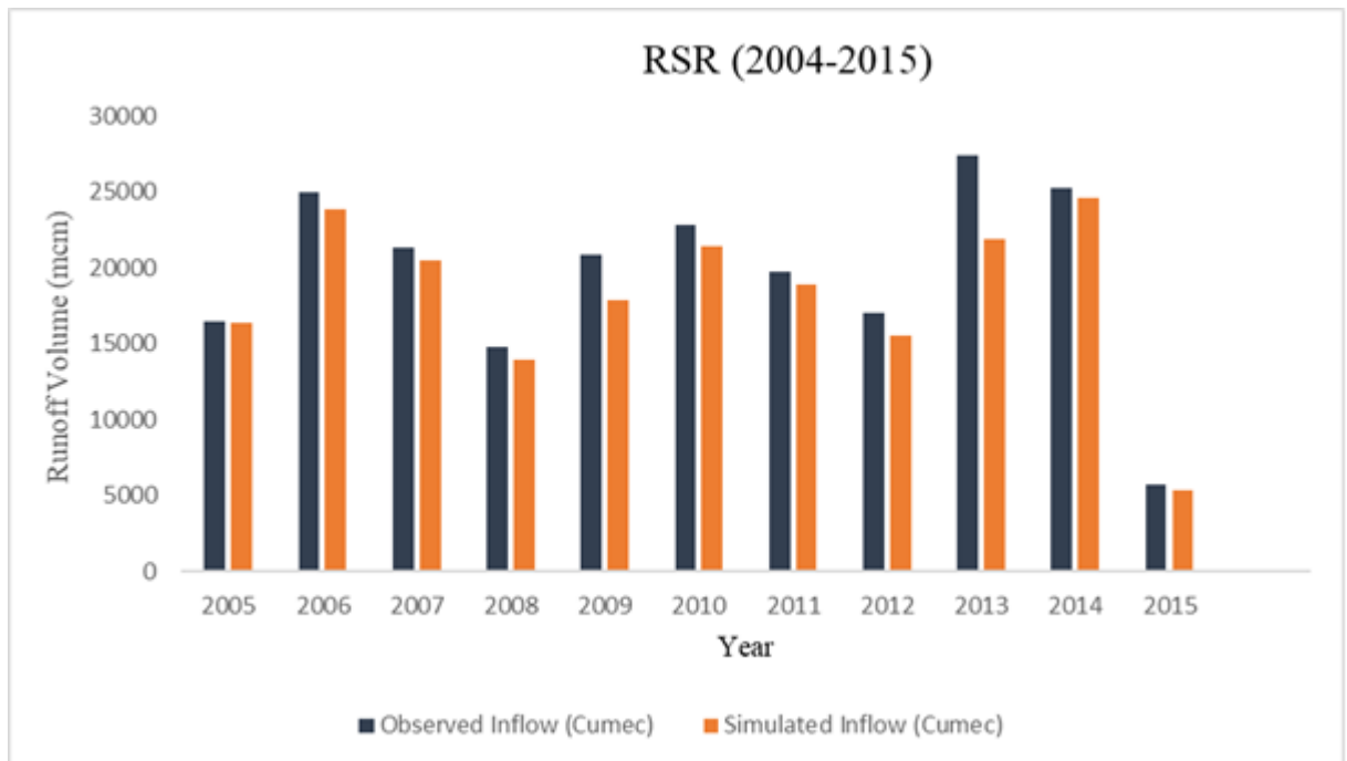
Figure 12: Observed and simulated monthly runoff volume during model calibration
