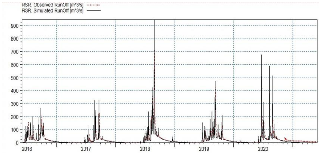
Figure 13: Observed and simulated runoff hydrograph during model validation
