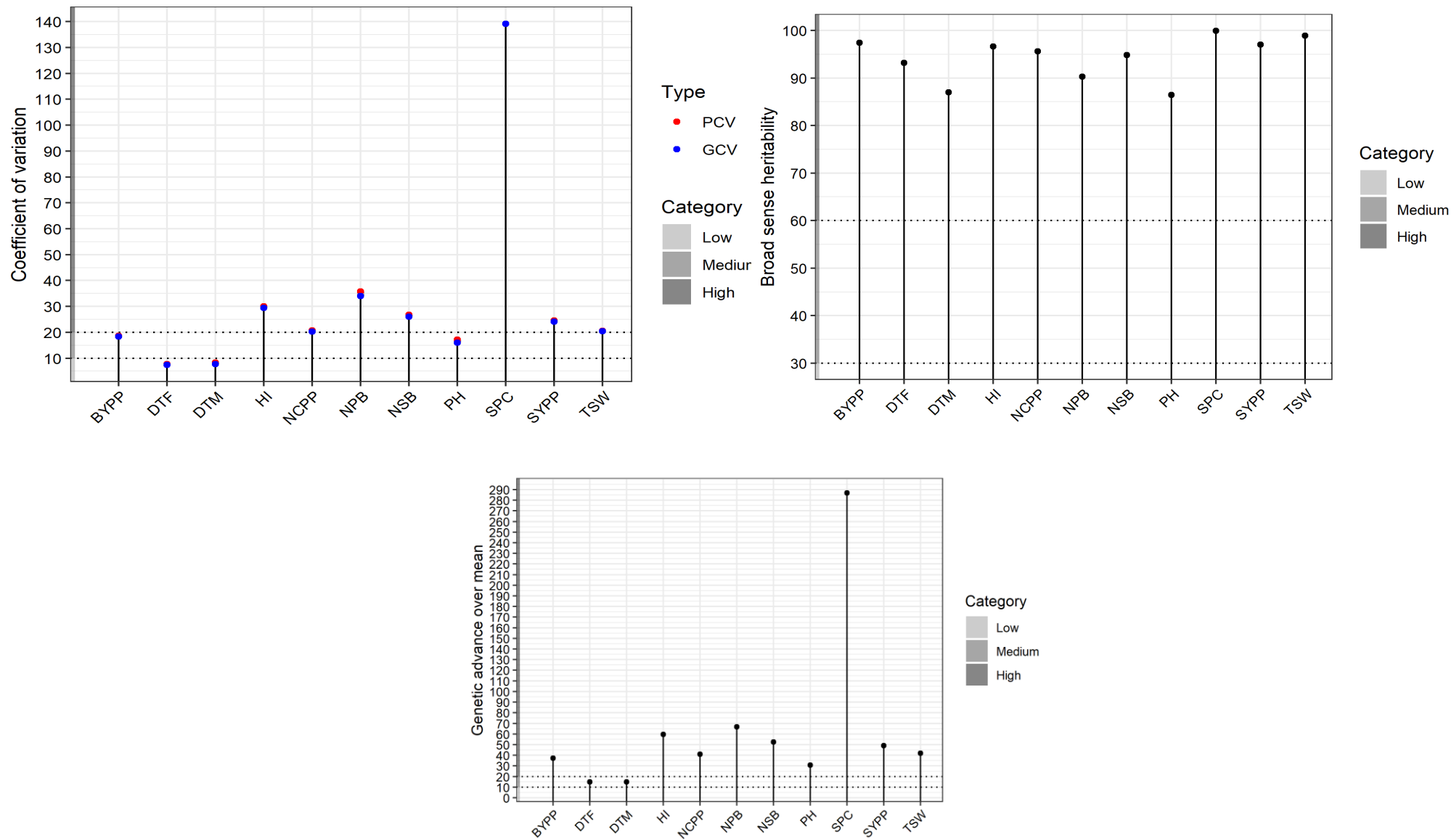
Fig.1 (a) Coefficient of variation for eleven traits showing high,medium, and low categories
