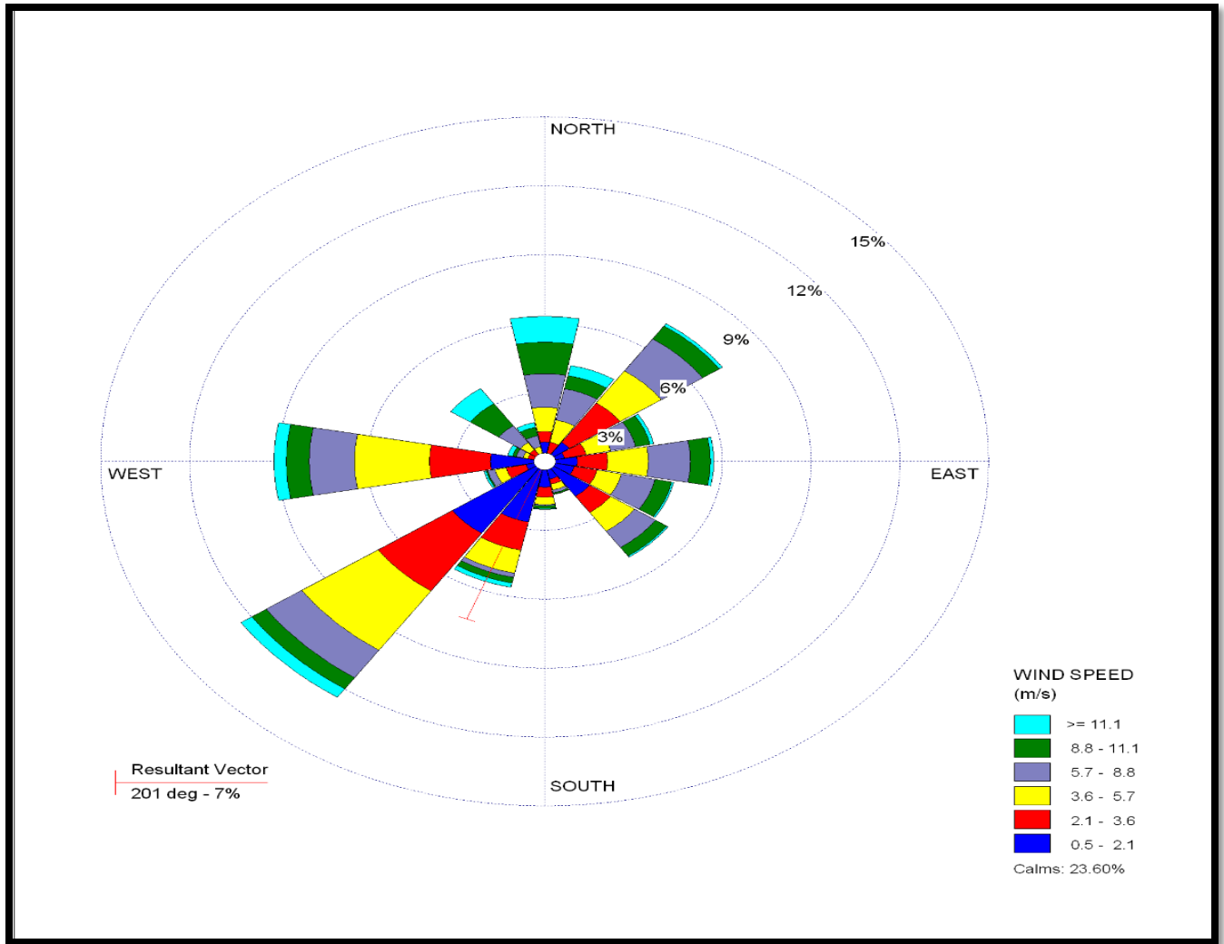
Figure 10: Windrose Map of study area during the sampling days.
