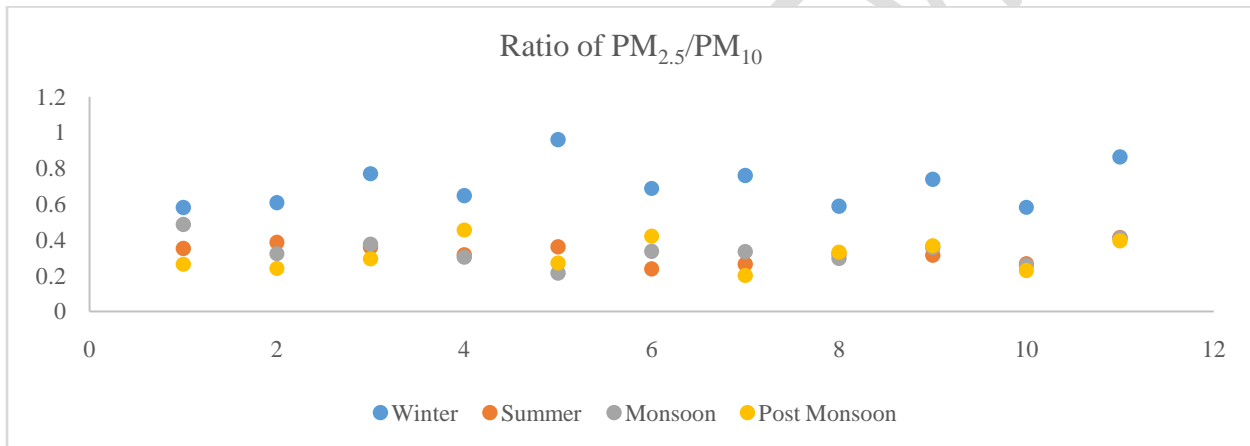
Figure 9: Seasonal Variation in the Ratio of PM 2.5 and PM 10
