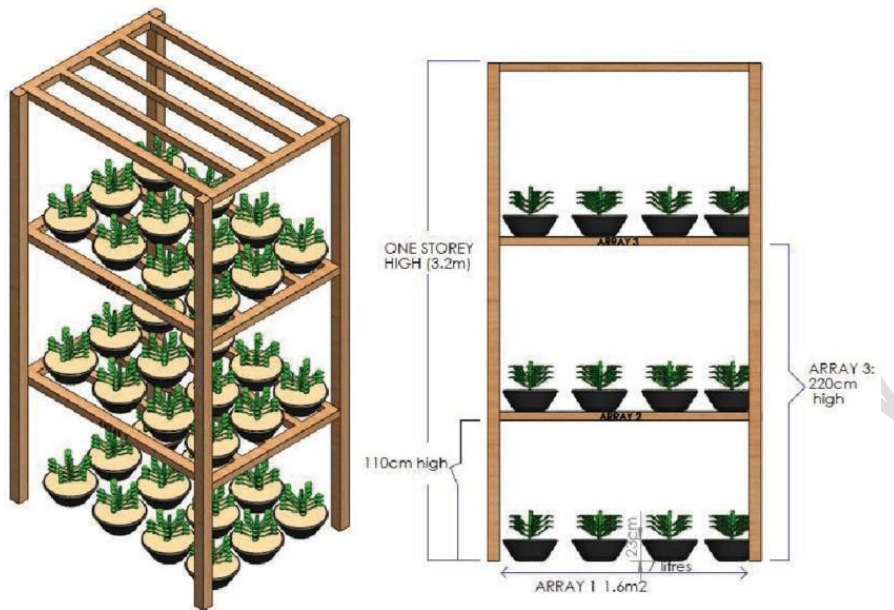
Figure 1: Schematic representation of a vertical farming system
