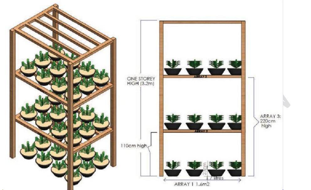
Figure 1: Schematic representation of a vertical farming system
