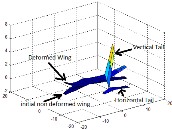
Figure 6-Airplane at trimmed condition – 224.6m/s, 10000 m, EA=0.00 c. Perspective.
