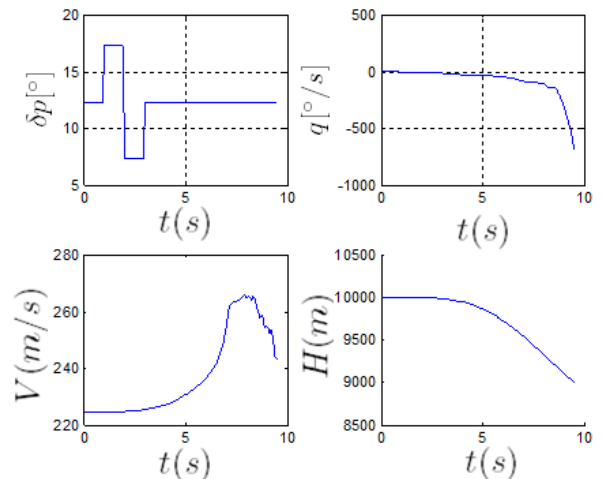
Figure 29b- Airplane with zero wing sweep, response to elevator doublet, V=224.6m/s, EA=-0.25c
