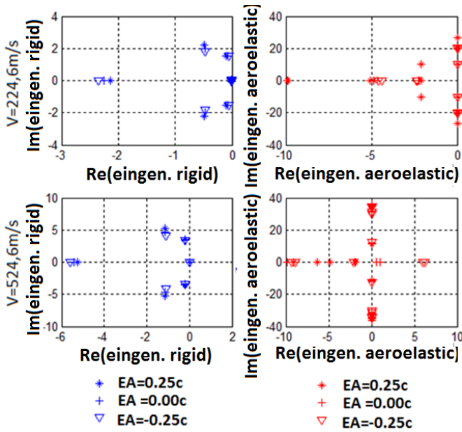
Figure5- Eigenvalues calculated for cases 1 to 6.
