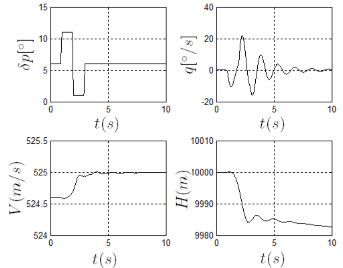
Figure 16- Airplane Response to one doublet of elevator, V=524.6m/s , EA=0.25 c .
