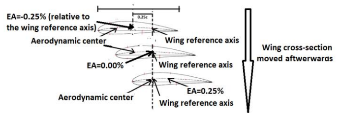
Fig.3 airfoil and reference axes
