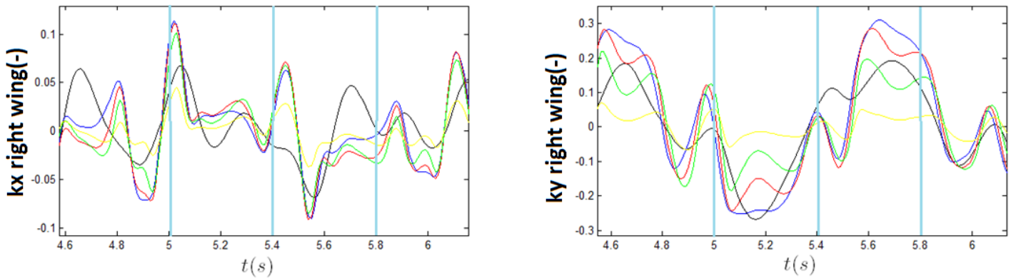
Figure 27-Phase difference between bending and twist deformations – Close view – Figure 21
