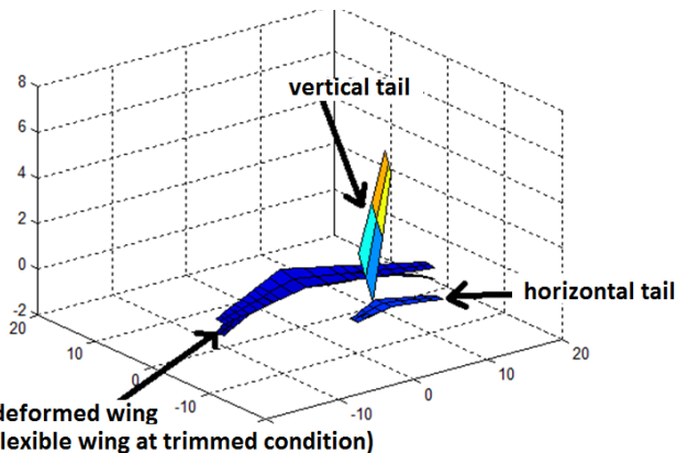
Figure 14- Airplane at trimmed condition – 524.6m/s, 10000 m, EA= 0.00 \%c ., perspective.
