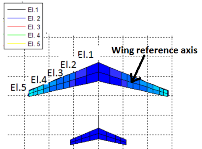
Fig.2 Structural elements on the wing [22]
