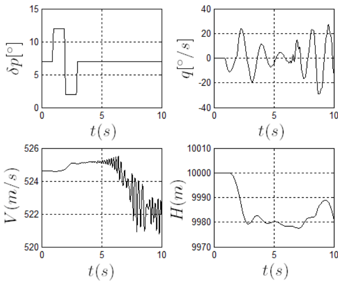
Figure 18–Airplane Response to one doublet of elevator, V=524.6\text{m/s} , EA= 0.00\text{ c}
