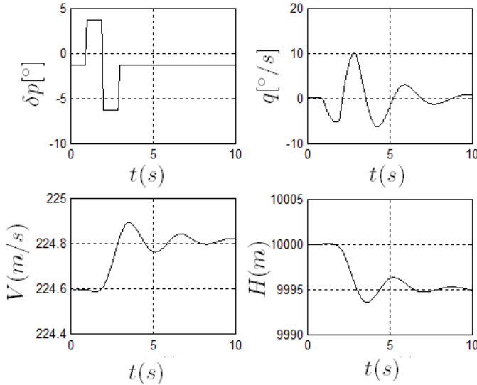
Figure 10–Airplane Response to one doublet of elevator, V=224.6m/s, EA= 0.00c
