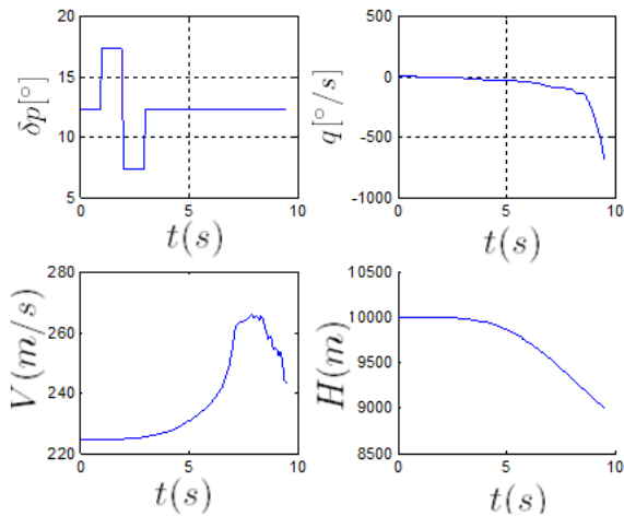
Figure 28b- Airplane with zero wing sweep, response to elevator doublet, V=224.6m/s, EA=0.00c.
