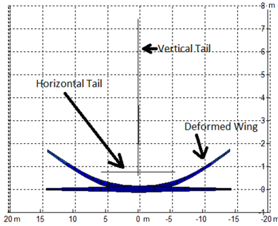
Fig.4 – Frontal view of airplane at trimmed condition.
