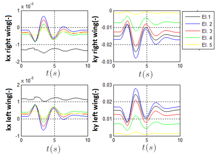
Figure 9-Bending and Twist Wing response to one doublet of elevator, V=224.6m/s, EA=0.25 %c
