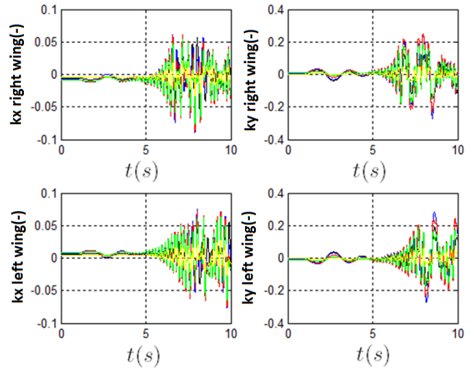
Figure 19– Bending and Twist Wing response to one doublet of elevator, V=524.6\text{m/s} , EA= 0.00\text{ c}
