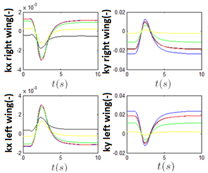
Figure 28c- Airplane with zero wing sweep, response to elevator doublet, V=224.6m/s, EA=0.00c
