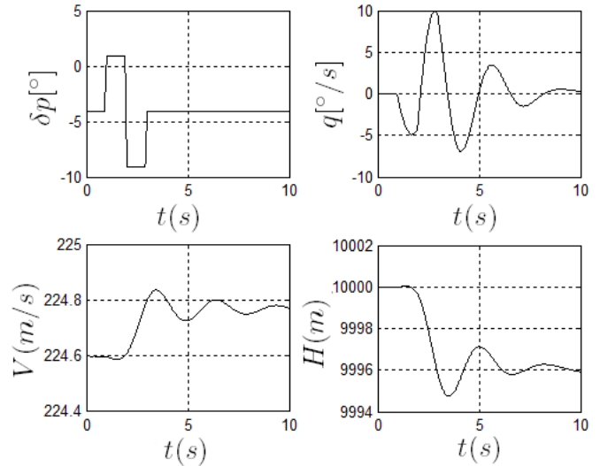
Figure 8-Airplane Response to one doublet of elevator, V=224.6m/s, EA=0.25 c
