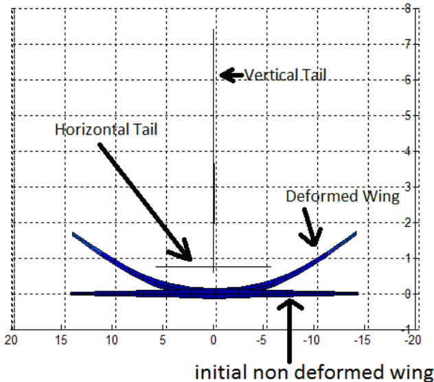
Figure 7-Airplane at trimmed condition – 224.6m/s, 10000 m, EA=0.00 c. , Frontal View
