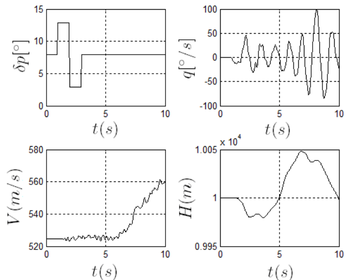
Figure 20 –Airplane Response to one doublet of elevator, V=524.6\text{m/s} , EA= -0.25\text{c}
