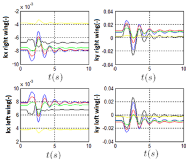
Figure 17– Bending and Twist Wing response to one doublet of elevator, V=524.6\text{m/s} , EA= 0.25\text{ c}
