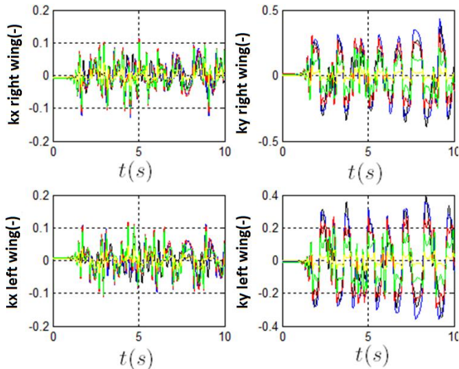
Figure 21- Bending and Twist Wing response to one doublet of elevator, V=524.6\text{m/s} , EA= -0.25 c
