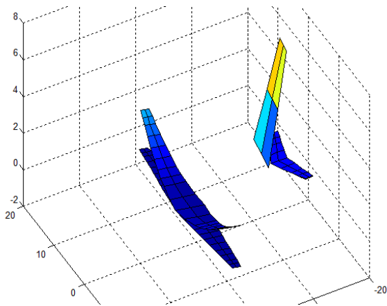
Figure 28a - Airplane with zero wing sweep trimmed at 224.6m/s and at 10000 m, EA=0.00c.
