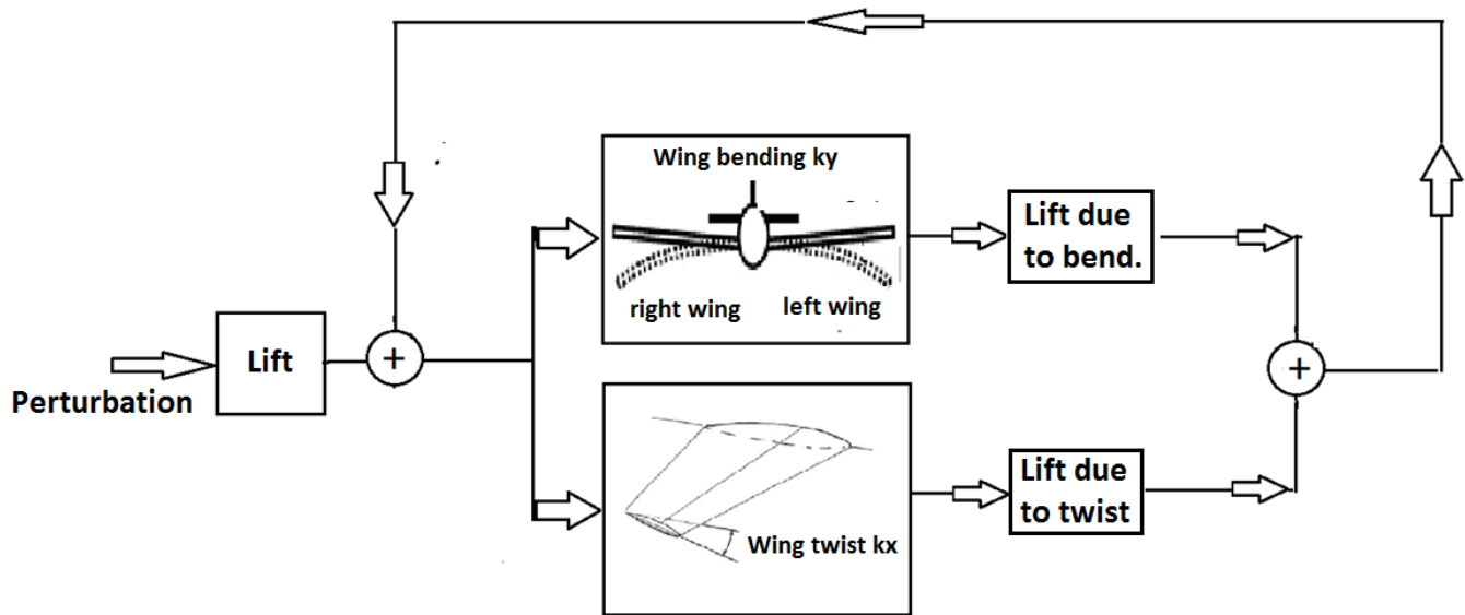
Figure 24 –Mechanism for amplification or damping of structural deformations
