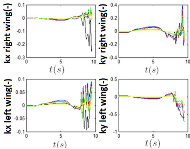
Figure 29c – Airplane with zero wing sweep, response to elevator doublet, V=224.6m/s, EA=-0.25c
