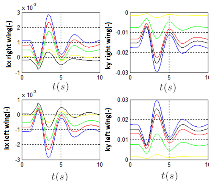
Figure 11- Bending and Twist Wing response to one doublet of elevator, V=224.6m/s, EA= 0.0 c
