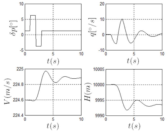
Figure 12 –Airplane Response to one doublet of elevator, V=224.6m/s, EA= -0.25c
