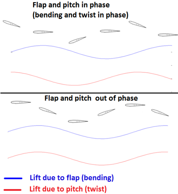
Figure 25- Example of phase difference between the pitch and flap movements
