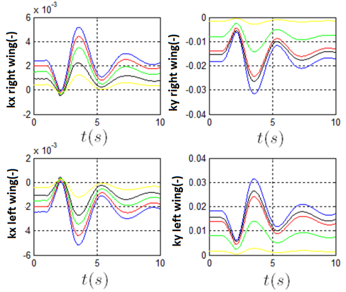
Figure 13 Bending and Twist Wing response to one doublet of elevator, V=224.6m/s, EA=-0.25c
