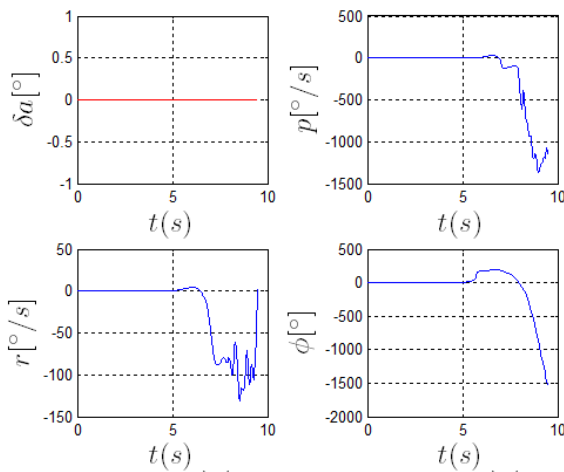
Figure 29d – Airplane with zero wing sweep, response to elevator doublet, V=224.6m/s, EA=-0.25c
