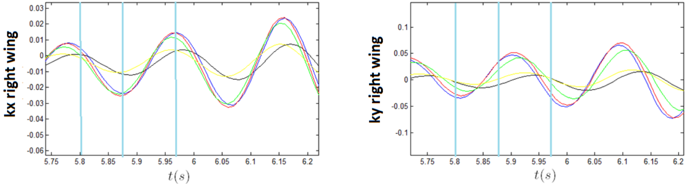
Figure 26- Phase difference between bending and twist deformations – Close view – Figure 19
