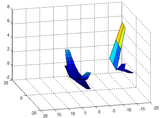
Figure 29a- Airplane with zero wing sweep trimmed at 224.6m/s and at 10000 m, EA=-0.25c.
