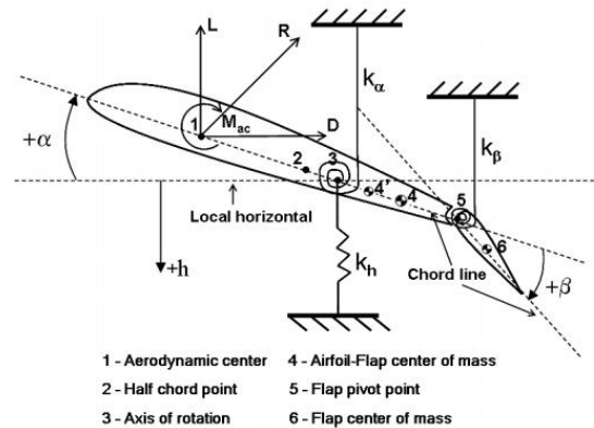
Figure 22- Two dimensional airfoil [18].
