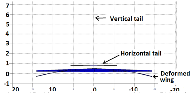
Figure 15- Airplane at trimmed condition – 524.6m/s, 10000 m, EA=0.00 c ., frontal View
