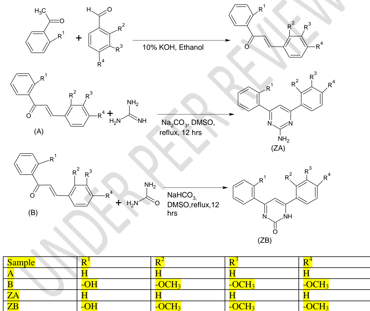
Figure 1: Synthesis of 1,3-diphenyl-2-propen-1-one (A-B) and derivatives (ZA-B)
