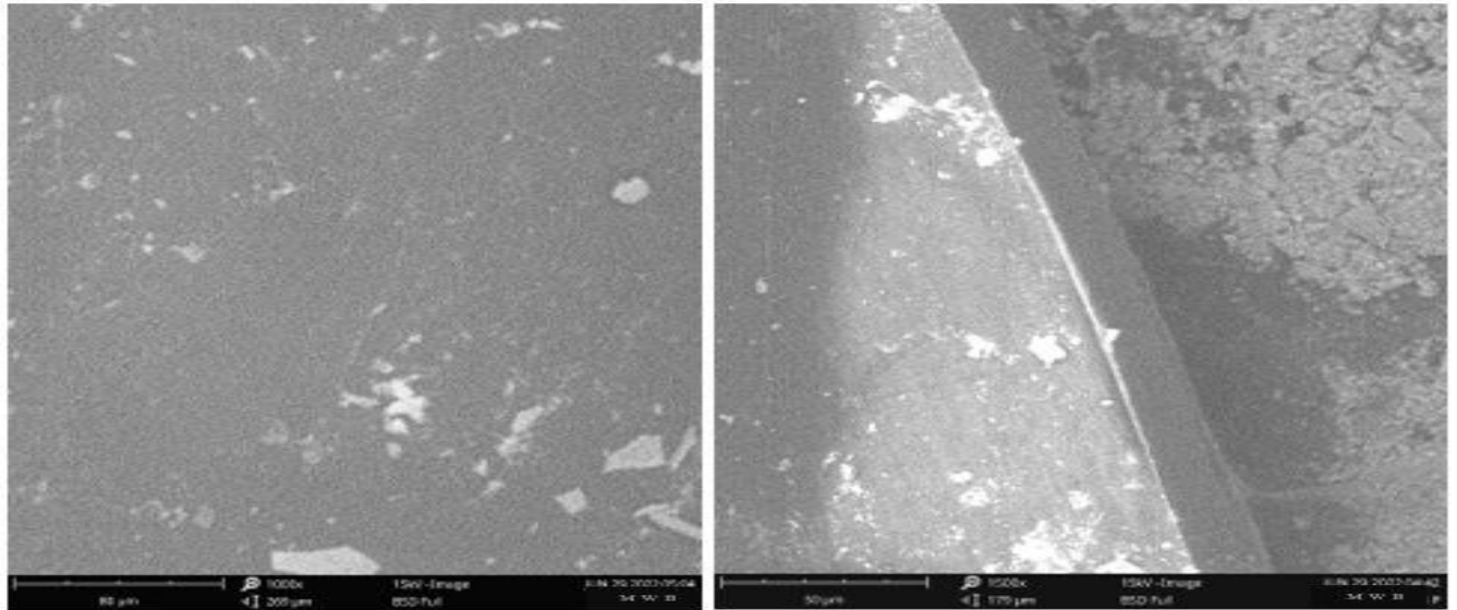
Plate 2: SEM Image of Bioplastic (PBS 1020) Before Test and 4 Months After in Marine Water
