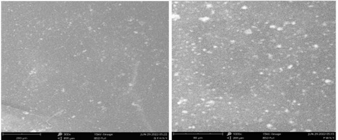
Plate 3:SEM Image of Synthetic Nylon 6 Before Test and 4 Months After in Fresh Water
