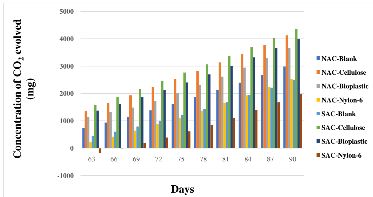
Figure 3: Carbon (iv) Oxide (CO 2 ) Evolution in Natural and Simulated Aqueous Conditions Across Ninety (90) Days
