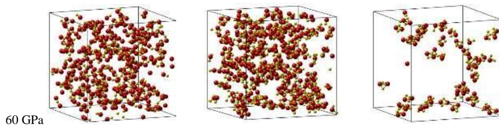
Fig. 5. Spatial distribution of \text{SiO}_x\text{-SiO}_y pairs connected through one, two, and three common oxygen atoms (core-, edge-, face-sharing) at pressures 0, 25, and 60 GPa. Here Si and O atoms are red, and yellow balls, respectively.
