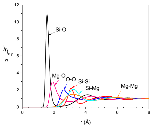
Fig. 1. The PRDFs of Si-O, Mg-O, O-O, Si-Si, Si-Mg, and Mg-Mg pairs in the Mg 2 SiO 2 model at 3500 K and 0 GPa.
